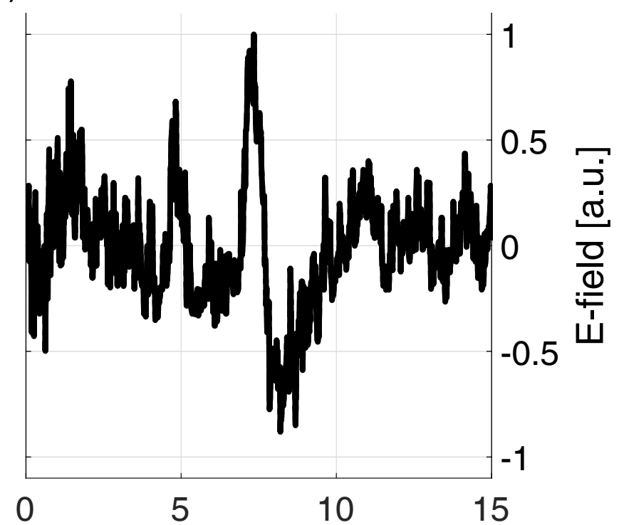
(f) Dust/waves/noise - TDS: other
