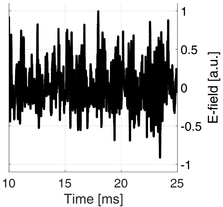
(i) Noise - TDS: other
