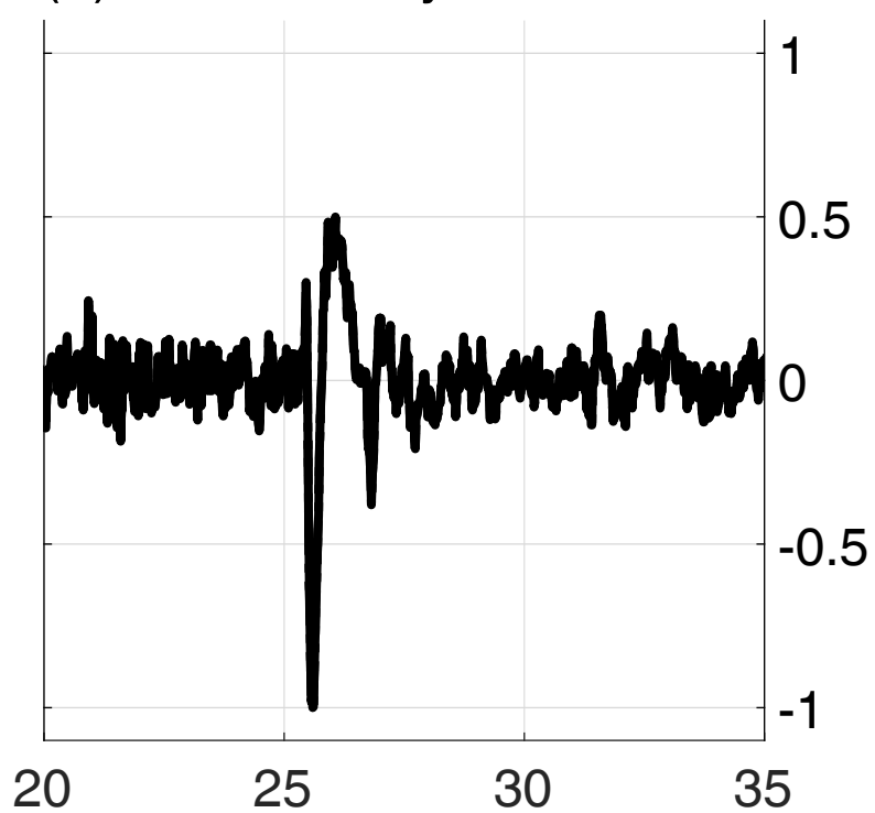
(e) Dust/solitary - TDS: other
