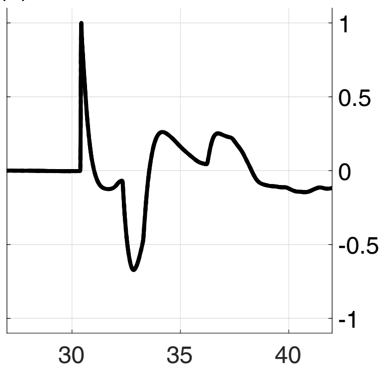
(b) Dust saturated - TDS: dust
