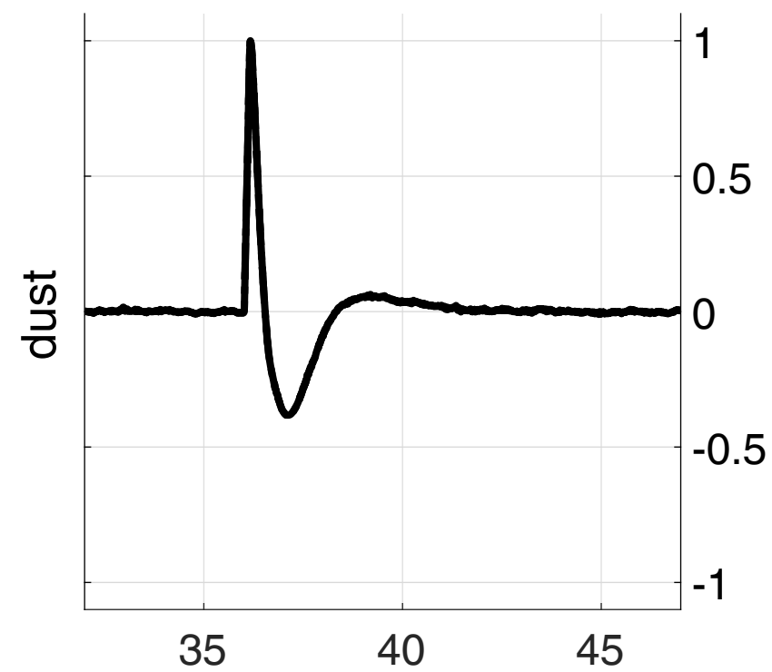
(a) Dust clean - TDS: dust
