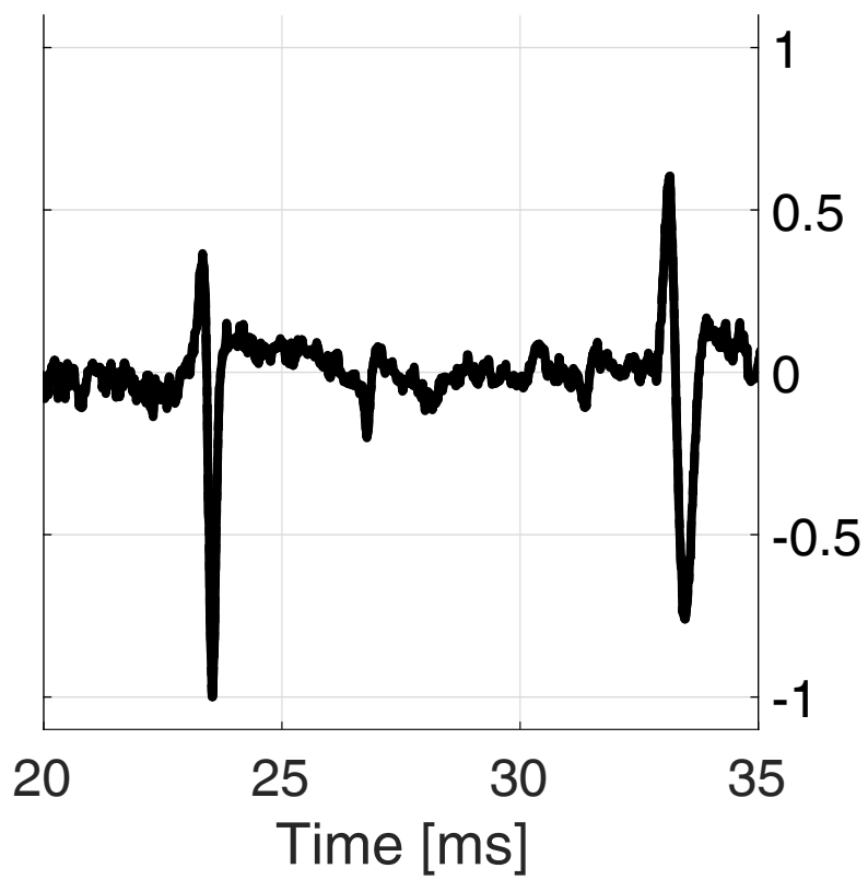
(h) Solitary - TDS: dust
