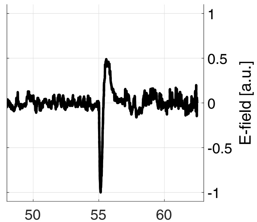
(c) Dust noisy - TDS: other
