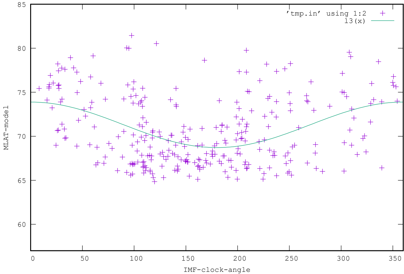
MLAT-vs-CLK-model
