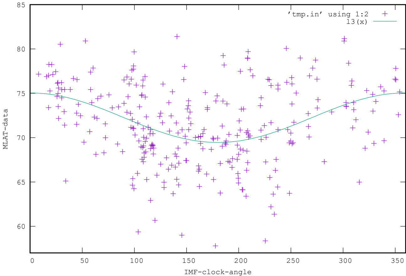
MLAT-vs-CLK-Data
