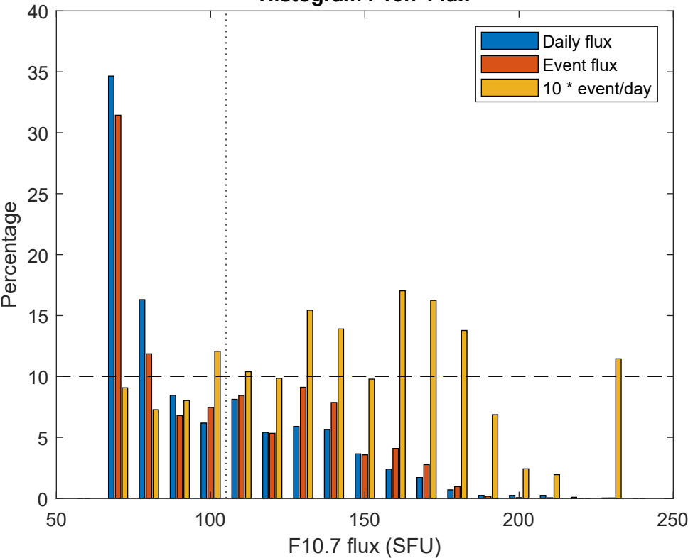
Histogram F10.7 Flux
