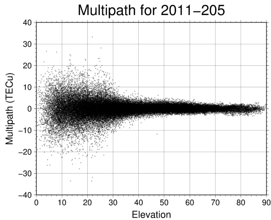
Figure 1. Multipath profile, in TEC units (“TECu”), for the Jason-2 satellite, derived from its GPS receiver data for day 205, 2011, using the differences between the SR and aligned SP.
