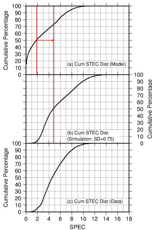
Figure 4. Cumulative distributions for the slant PEC (SPEC) values (in TEC units) from (a) PIM (for the same lines of sight as the data samples); (b) PIM, with added Gaussian noise, having a standard deviation of 0.75 TEC units; and (c) measured, calibrated SPEC data. The vertical red lines indicate the shift of the median of the cumulative distribution for the PIM values, induced by the noise tail at the low end of the distribution.
