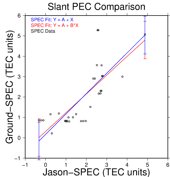
Figure 9. SPEC comparisons for ground-based GPS receivers (Ground-SPEC) versus the Jason-2 GPS receiver (Jason-SPEC) (circles), with two alternative linear fits: ( Y = A + X ) (blue) and ( Y = A + B \cdot X ) (red), both indicating intercepts of about 0.24 TEC units.
