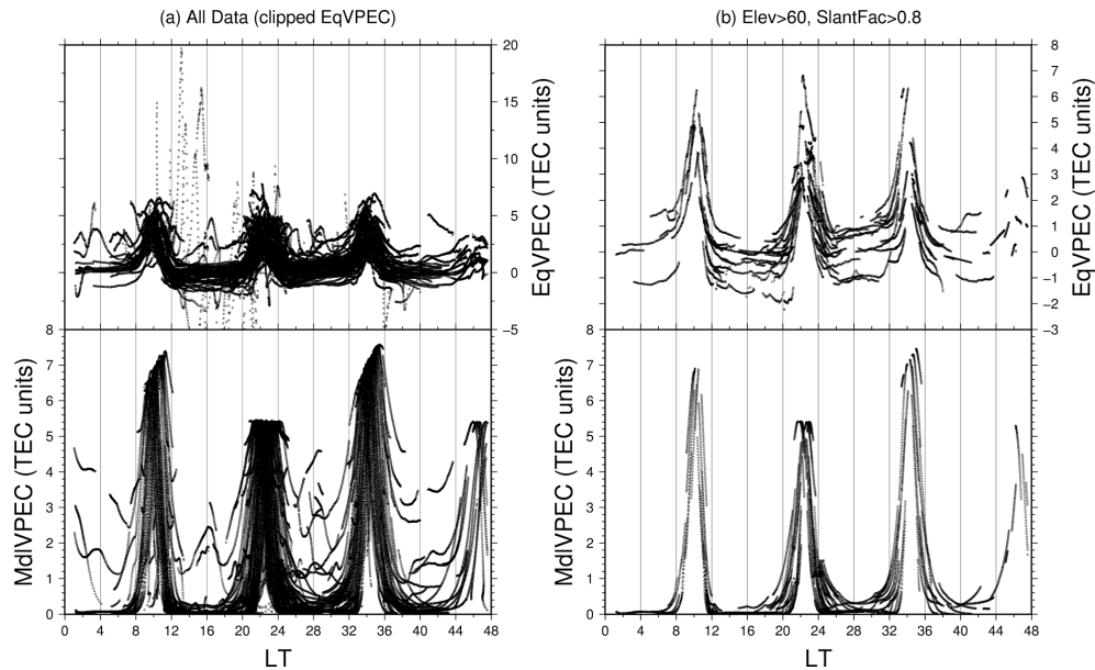
Figure 5. (a) PIM VPEC (MdlVPEC) and equivalent vertical measured PEC (EqVPEC) versus local time (LT) for all data samples (display limited from -5 TEC units for EqVPEC). The minimum EqVPEC value is nearly -36 TEC units, arising from small values for the ratio (SlantFac) of model slant PEC (MdlSPEC) to model equivalent vertical PEC (MdlVPEC). (b) MdlVPEC and EqVPEC versus LT for data subset, selected by 60^\circ \leq \text{Elevation} \leq 90^\circ and 0.8 \leq \text{SlantFac} .
