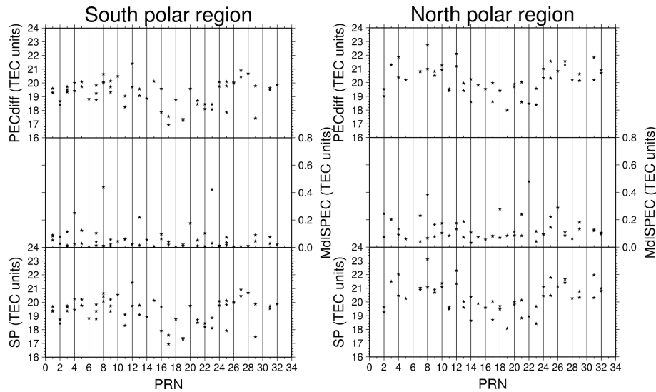
Figure 3. Comparisons of minimum Jason-2 uncalibrated GPS SPEC (SP) values with minimum PIM SPEC (MdlSPEC) for contiguous GPS satellite segments in each polar region, with the corresponding differences PECdiff = SP - MdlSPEC , for each GPS PRN number.
