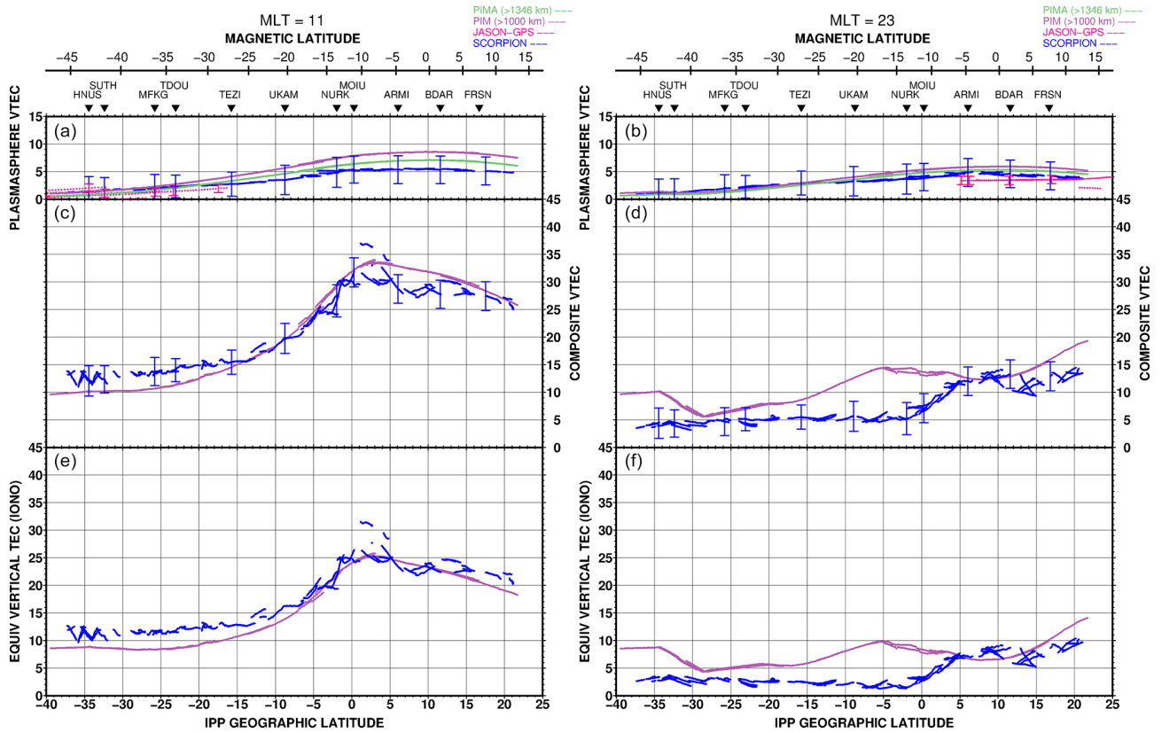
Figure 7. Latitudinal vertical TEC profiles (in TEC units) separately for the ionosphere (e, f) and plasmasphere (a, b) (for an ionosphere–plasmasphere boundary at 1000 km), with the composite (ionosphere plus plasmasphere) vertical TEC (c, d), for the SCORPION and PIM results and for the plasmasphere only for the Jason-2 results (with a base altitude of 1346 km) for magnetic local times 11:00 (a, c, e) and 23:00 (b, d, f). The corresponding PIM profiles are displayed for a 1000 km boundary for the ionosphere only (e, f) and as the upper PIM profile (“PIM (>1000 km)”) for the plasmasphere, while the lower PIM plasmasphere profile (“PIMA (> 1346 km)”) corresponds to an alternative boundary altitude of 1346 km for comparison with the Jason-2 values.
