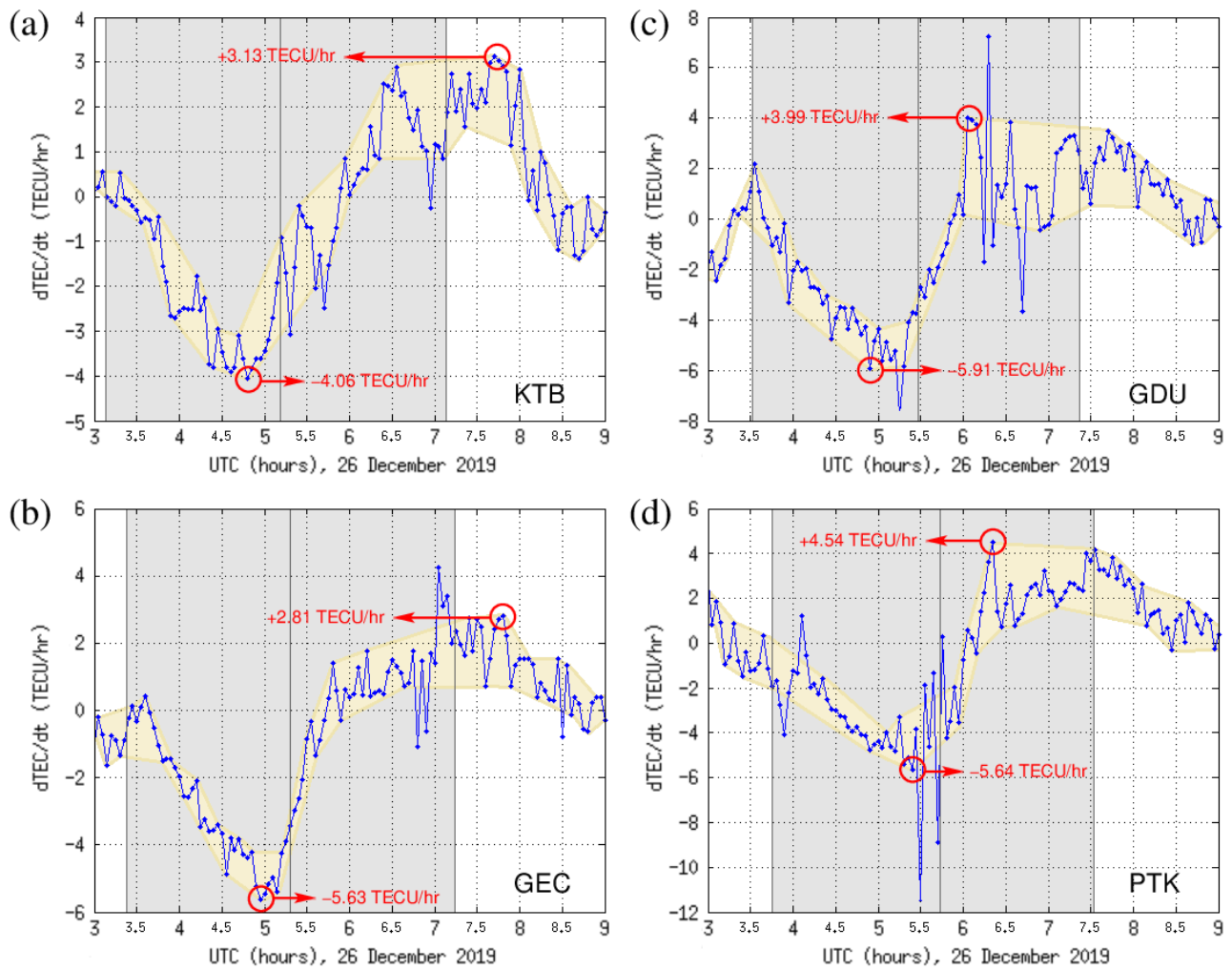
Figure S2. Magnified time series plots of the TEC time derivative ( dTEC/dt ) around the solar eclipse period over the 4 designated check points (KTB, GEC, GDU, and PTK). The solar eclipse period is indicated with gray bands, and the general dTEC/dt trend (bypassing large spikes) is shown as yellow bands. Minimum and maximum values in the dTEC/dt trend are marked accordingly on the plots.
