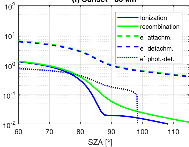
(f) Sunset - 80 km
