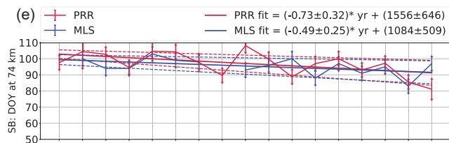
Mesosphere - Summer Length (M-SL)
