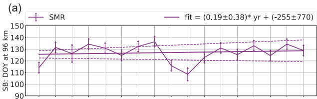
Mesosphere and Lower Thermosphere - Summer Length (MLT-SL)
