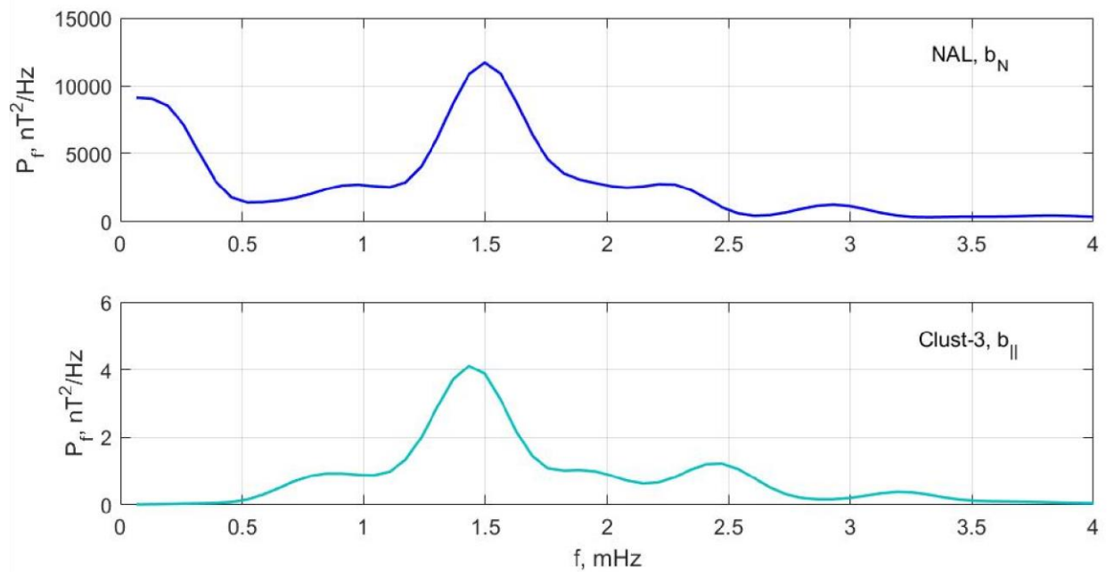
Figure S1. PSD spectra of non-filtered time series (start UT =15:44). NAL ground-based magnetic data; Cluster 3 field aligned component.
