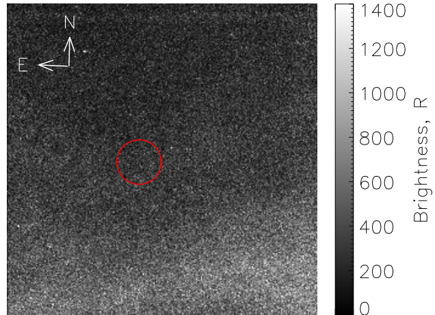
(b) ASK3 OI 777.4 nm
