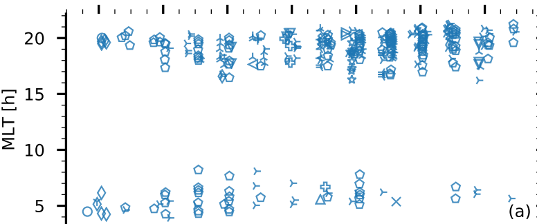
SSUSI F17 - EISCAT Tromsø UHF IS radar
