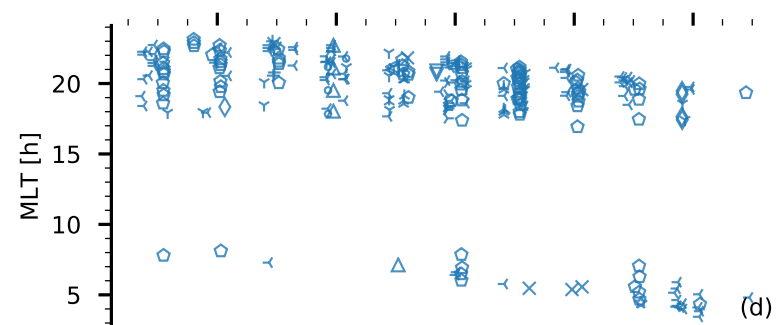
SSUSI F18 - EISCAT Tromsø UHF IS radar
