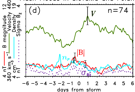
SOLAR WIND 1963–2019 Flash Floods in Slovakia and Poland
