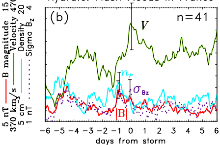
SOLAR WIND 1963–2002 Hydrate: Flash Floods in France
