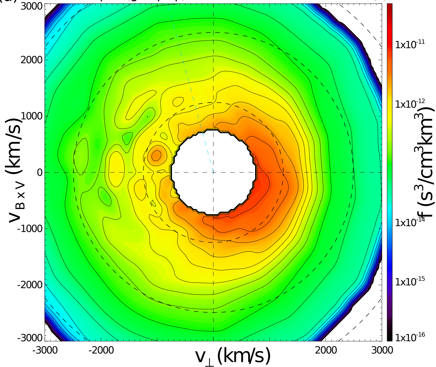
(a) THEMIS b ptibf (gsm perp) 2008-03-01/01:55:19 -> 01:55:31 (4)
