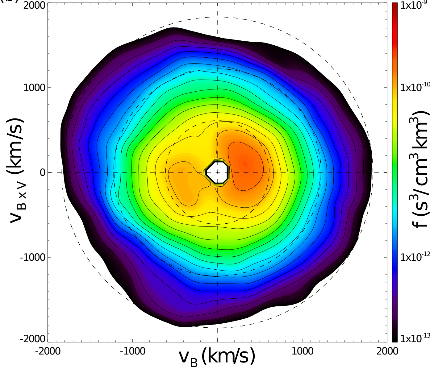
(b) THEMIS b ptirf (gsm BE) 2014-11-06/21:40:52 -> 21:41:03 (3)
