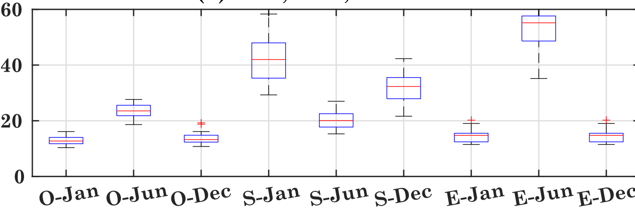
(b) TEC, 2013, 40°N/15°E
