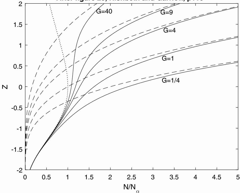
After figure 28, Rishbeth and Garriott, p116
