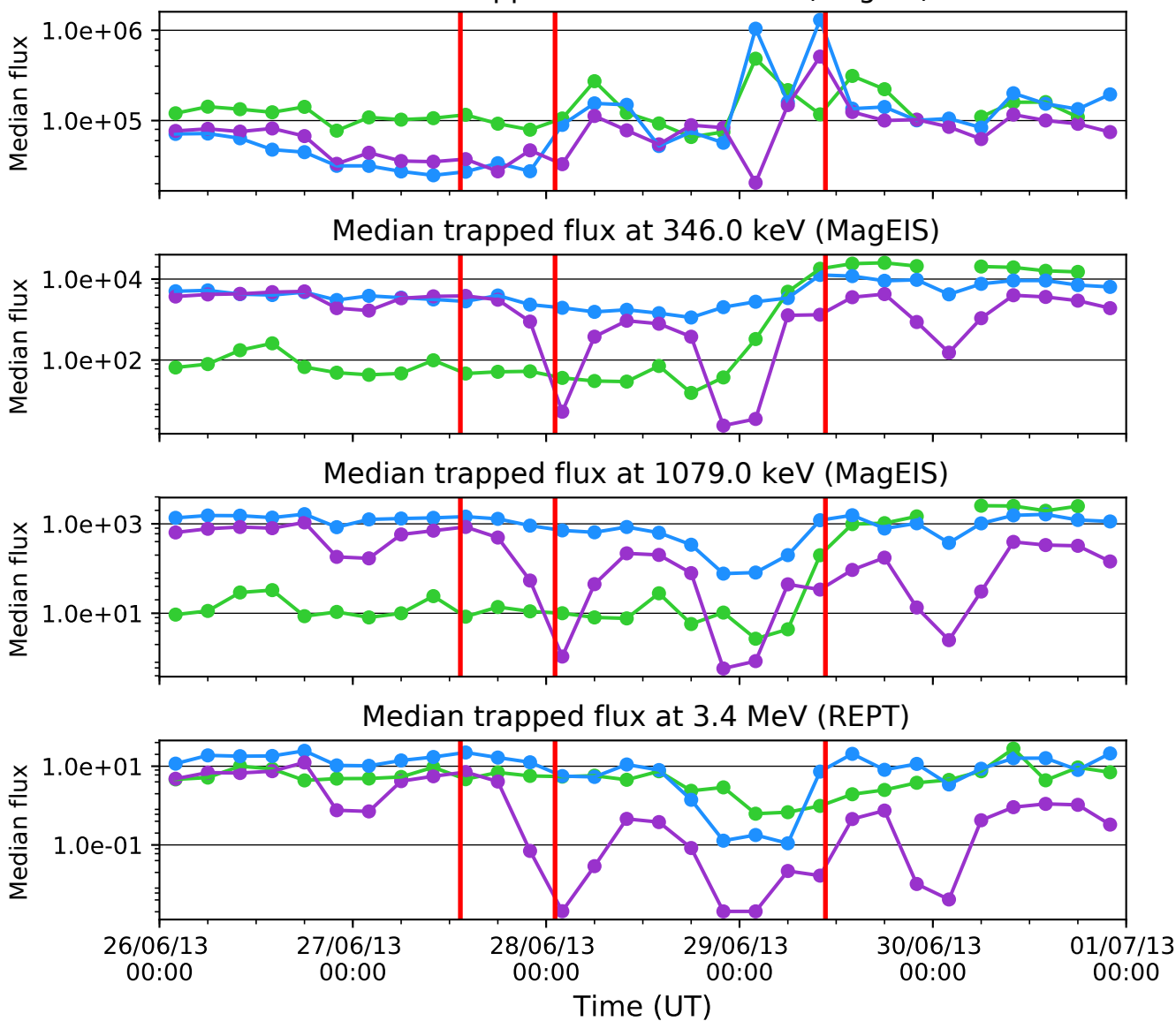
Median trapped flux at 33.0 keV (MagEIS)
