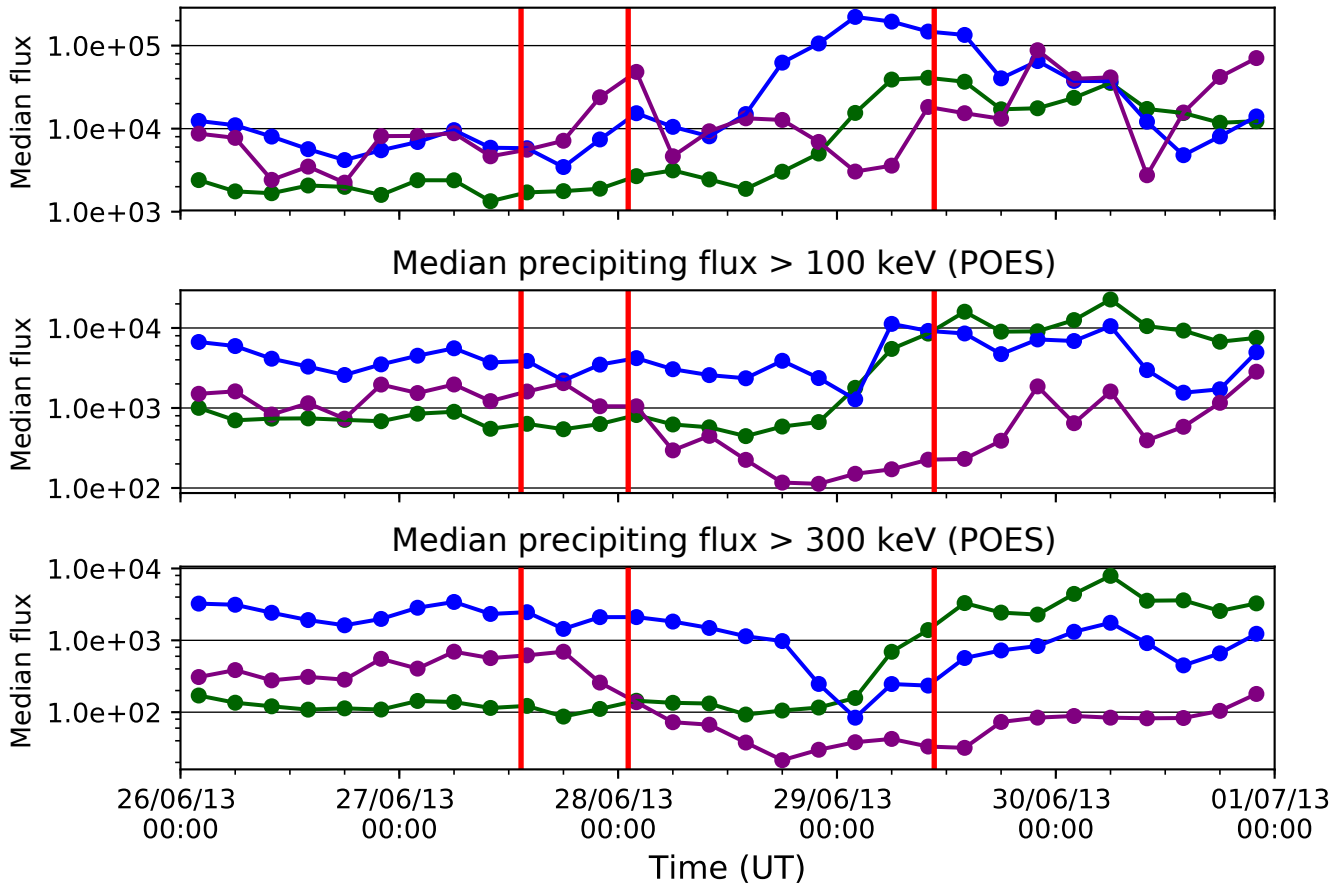
Median trapped flux at 33.0 keV (MagEIS)
