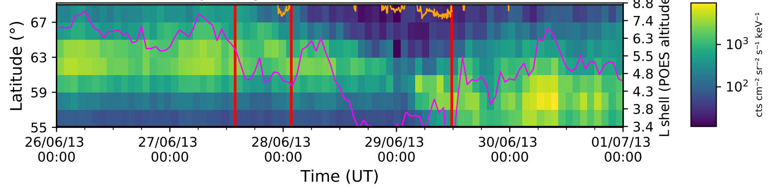
Trapped electron flux at 33.0 keV (MagEIS)
