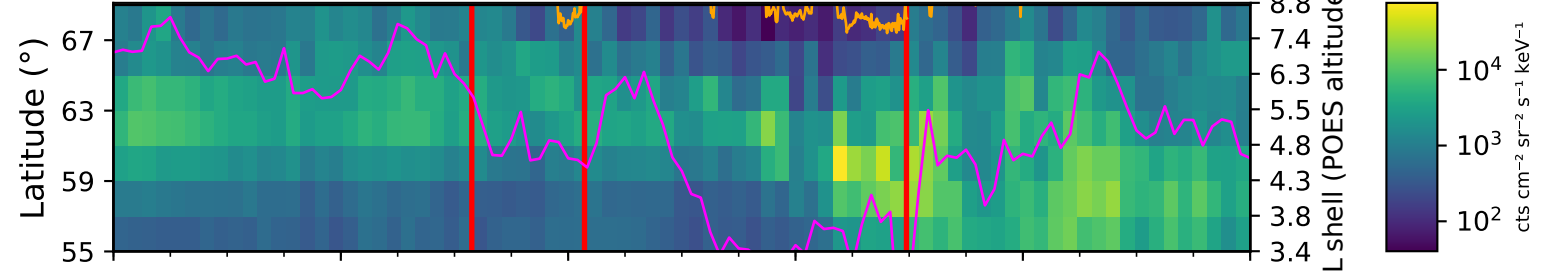
Precipitating electron flux > 300 keV (POES)
