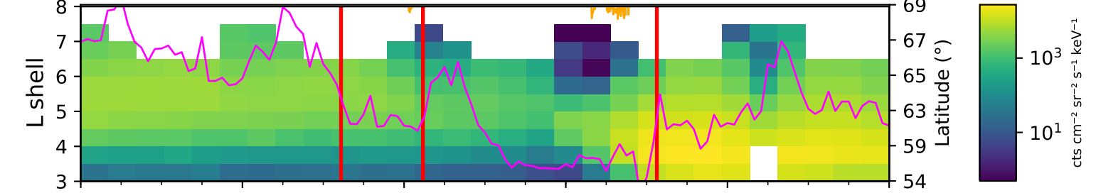
Trapped electron flux at 1079.0 keV (MagEIS)
