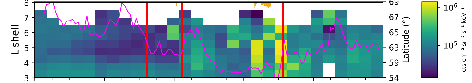
Trapped electron flux at 346.0 keV (MagEIS)
