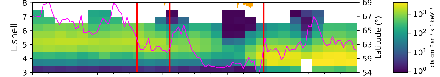
Trapped electron flux at 3.4 MeV (REPT)
