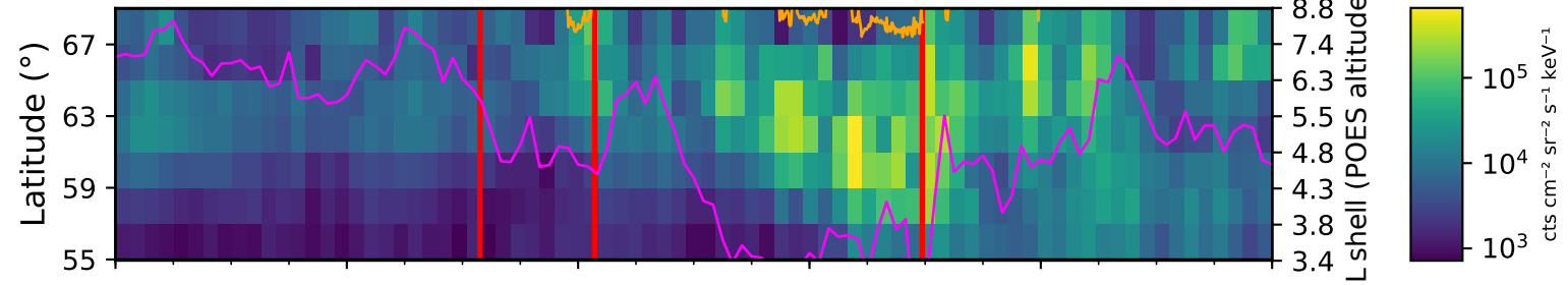
Precipitating electron flux > 100 keV (POES)
