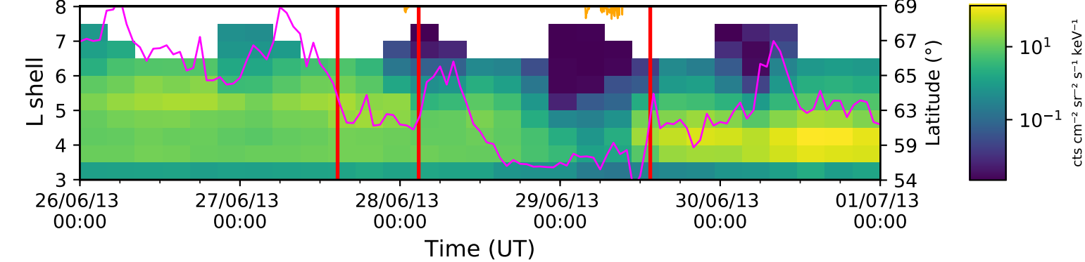
Trapped electron flux at 3.4 MeV (REPT)
