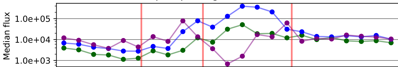
Median precipitating flux > 100 keV (POES)
