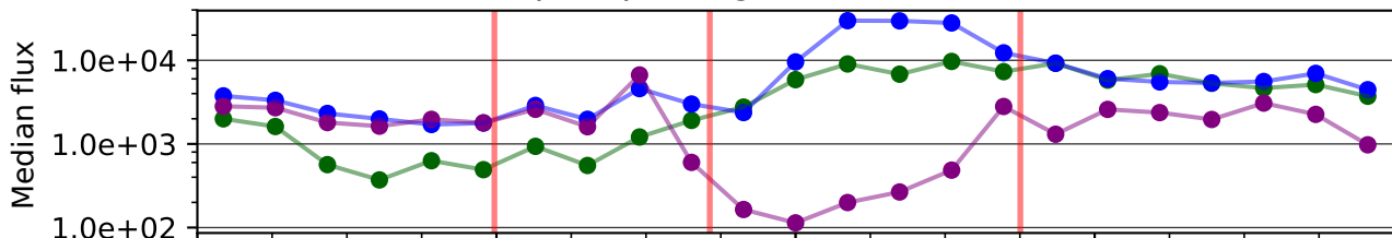
Median precipitating flux > 300 keV (POES)
