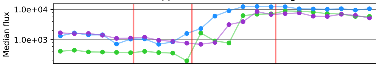
Median trapped flux at 1079.0 keV (MagEIS)
