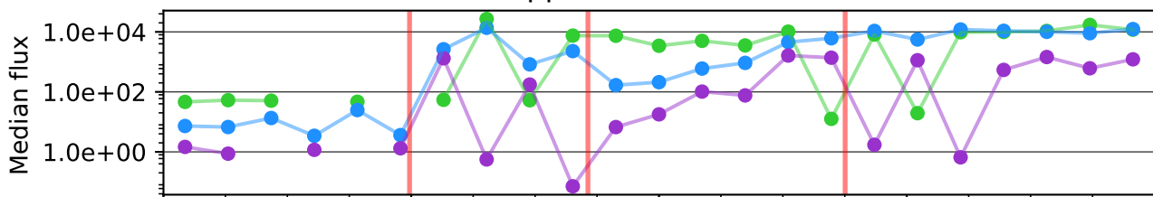
Median trapped flux at 3.4 MeV (REPT)
