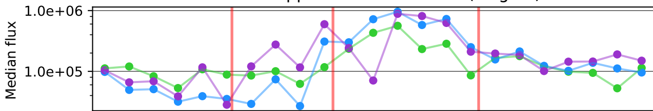
Median trapped flux at 346.0 keV (MagEIS)
