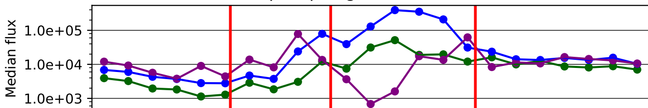
Median precipitating flux > 100 keV (POES)
