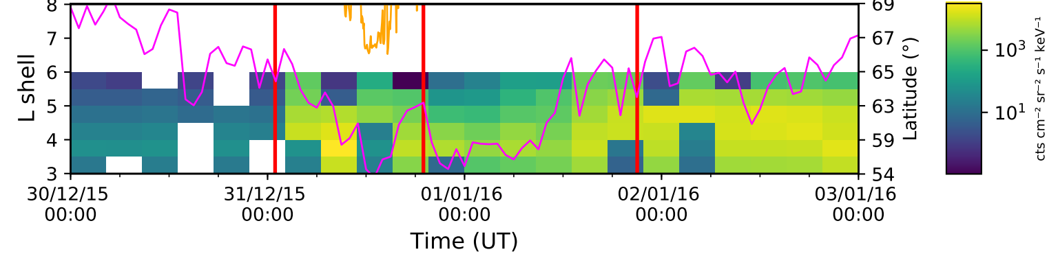
Trapped electron flux at 3.4 MeV (REPT)
