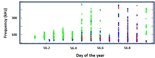
Figure 4. Vertical lines indicate the occurrence of the frequency-banded emissions observed on 25 February 2010. Those events were recorded on the night side of Earth with a time interval of about 1 h 35 min. Green, blue and red specify, respectively, three power level intervals, i.e. 10^{-3} – 0.7 , 0.7 – 10 and 10 – 10^{+4} \mu\text{V m}^{-1} \text{Hz}^{-1/2} .
