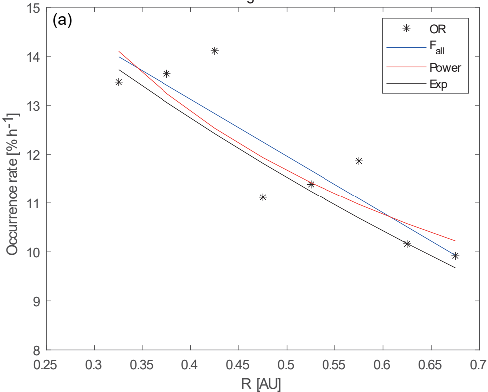
Linear magnetic holes
