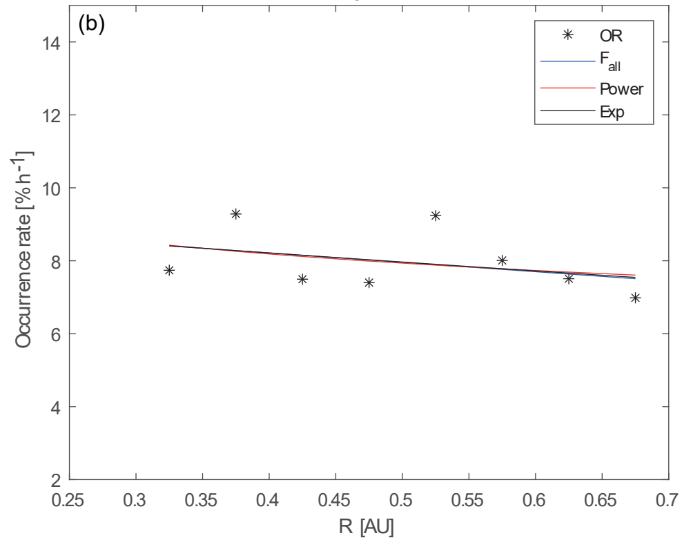
Pseudo magnetic holes
