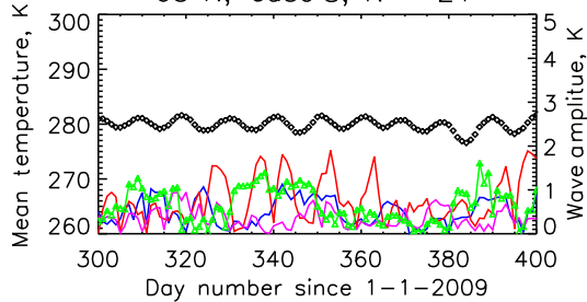
65°N, case 9, N = 21
