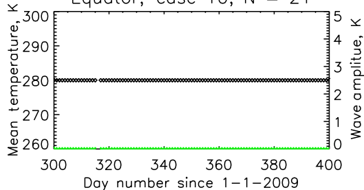
Equator, case 10, N = 21
