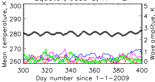
Equator, case 9, N = 21
