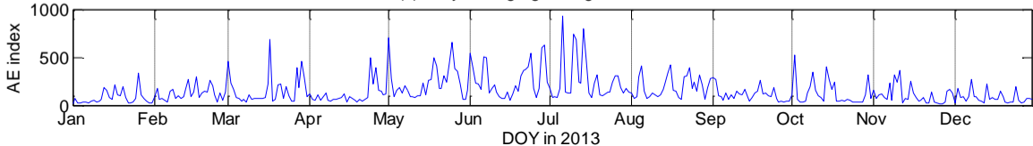
(c) Daily average geomagnetic AE index
