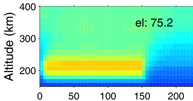
Modelled Te
