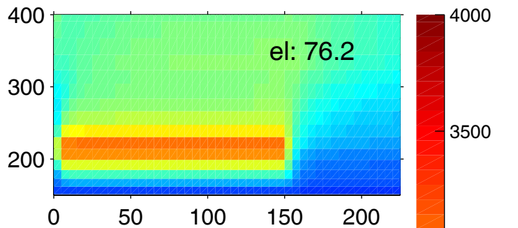
Modelled Te
