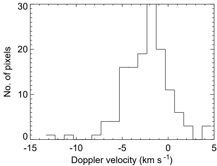
C II
