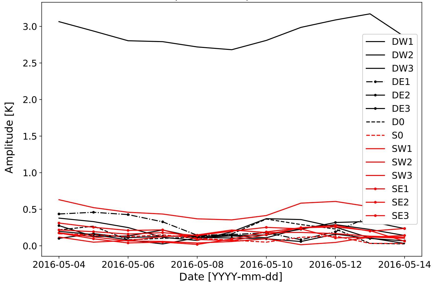
Tidal temperature components at 45 km
