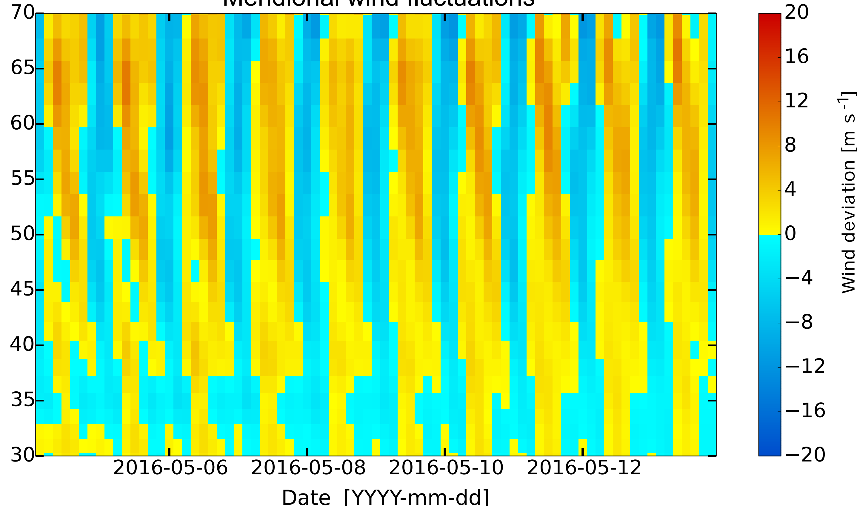
Meridional wind fluctuations
