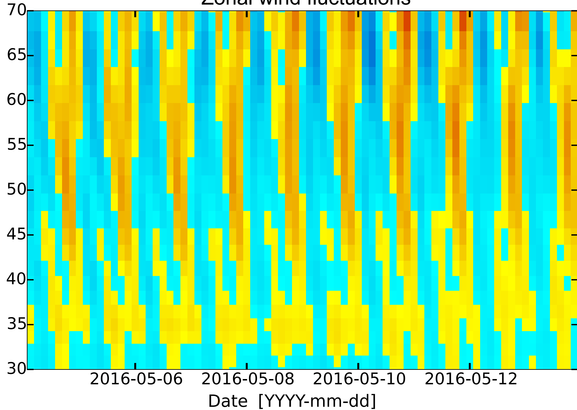
Zonal wind fluctuations
