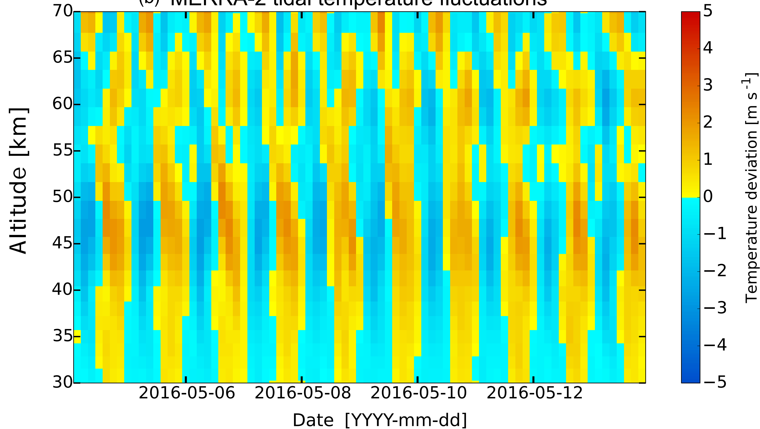
(b) MERRA-2 tidal temperature fluctuations
