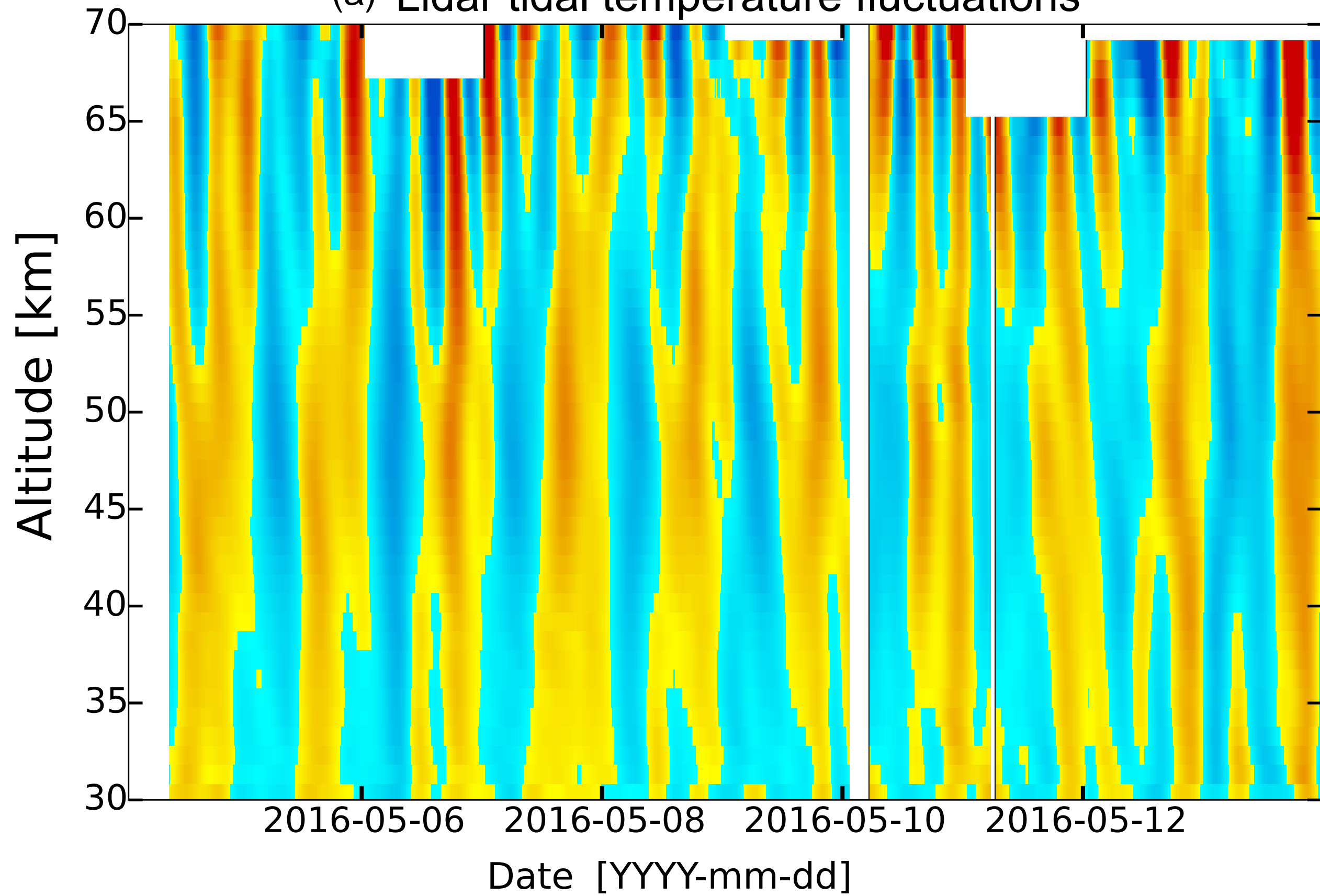
(a) Lidar tidal temperature fluctuations
