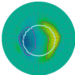
(b) July 16, 03:00 0.5 R_E
