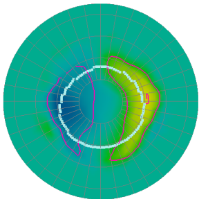
(a) July 16, 01:00 0.5 R_E
