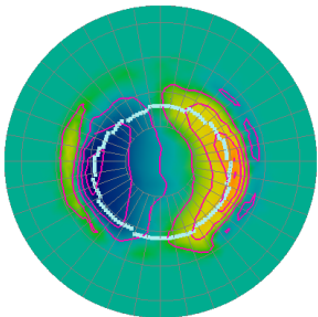
(c) July 16, 01:00 0.25 R_E
