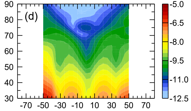
log10(Varia of recon_GWMF) (Pa 2 )
