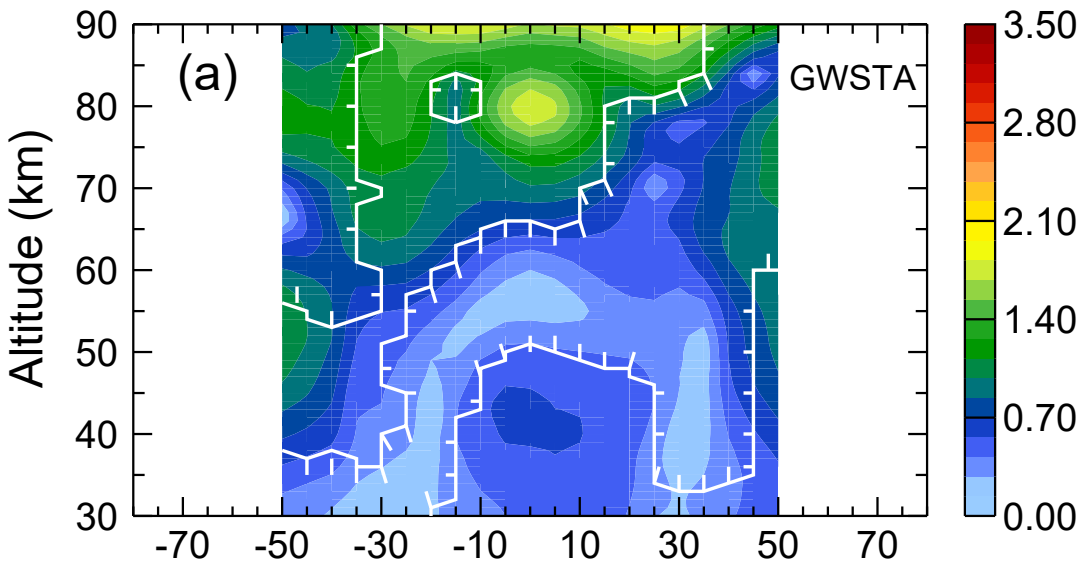
Spectral amplitudes (K) QBO
