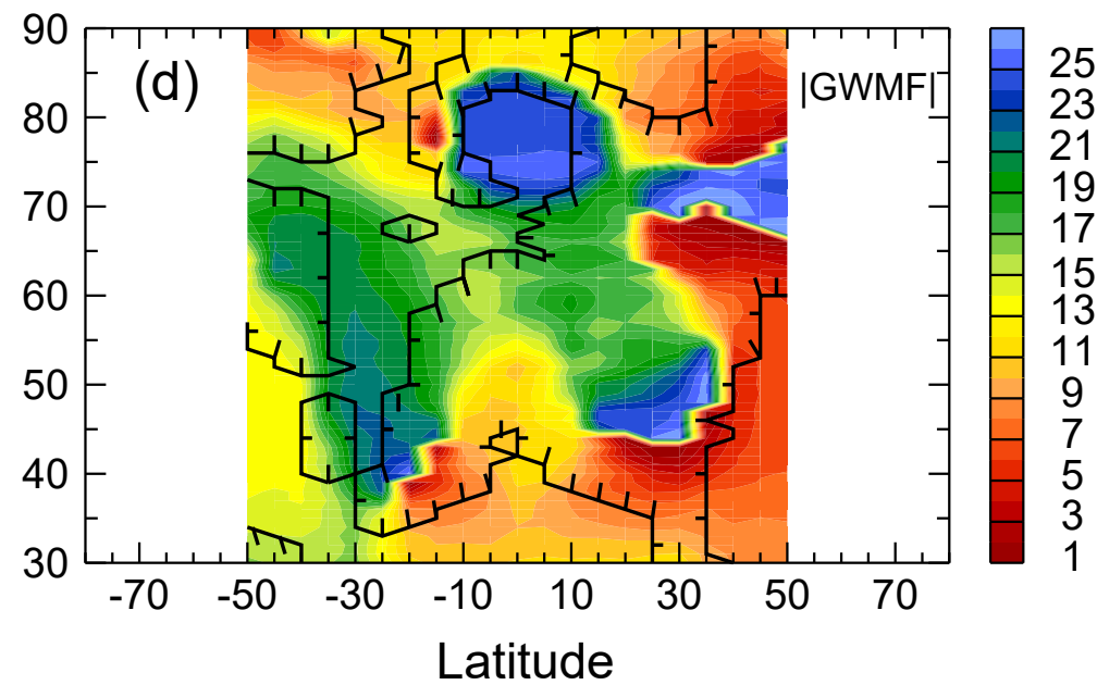
Phase QBO
