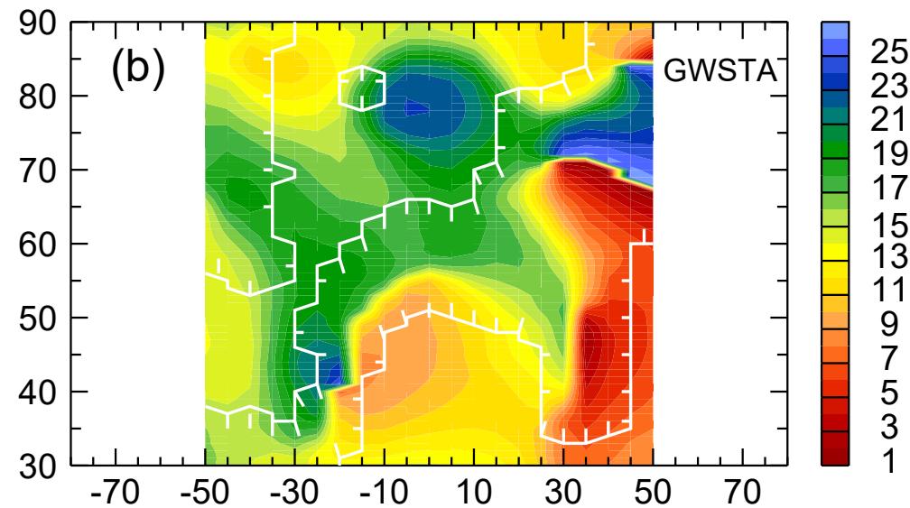
Phase QBO
