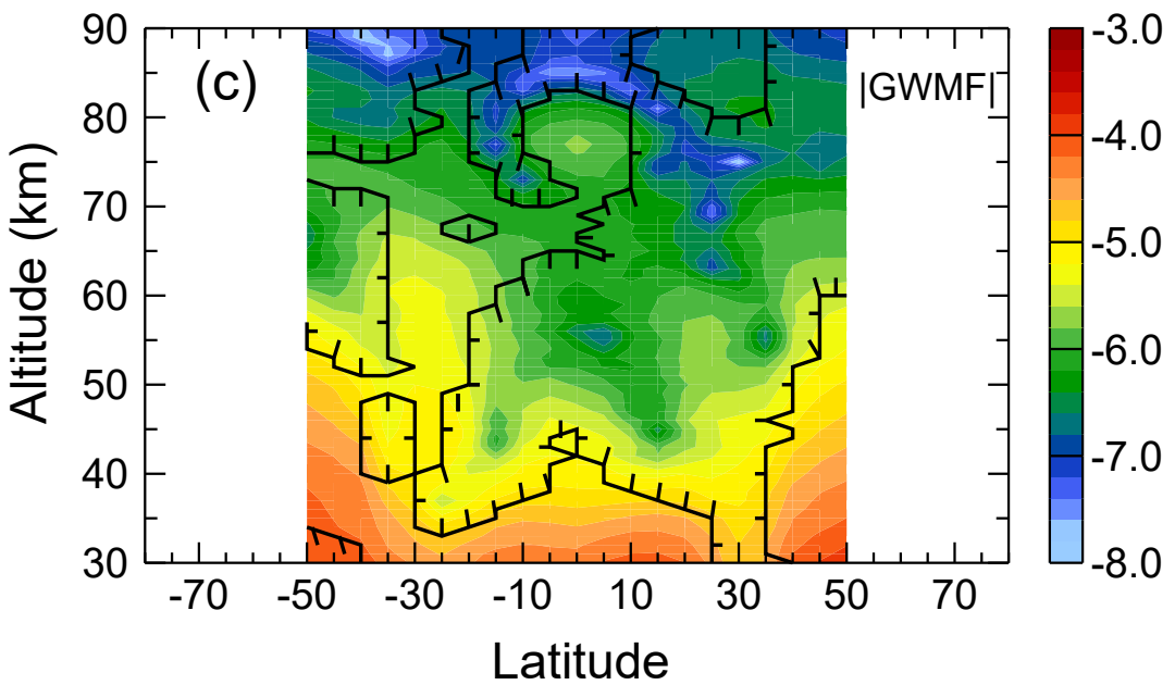
Spectral amplitudes (log10Pa) QBO
