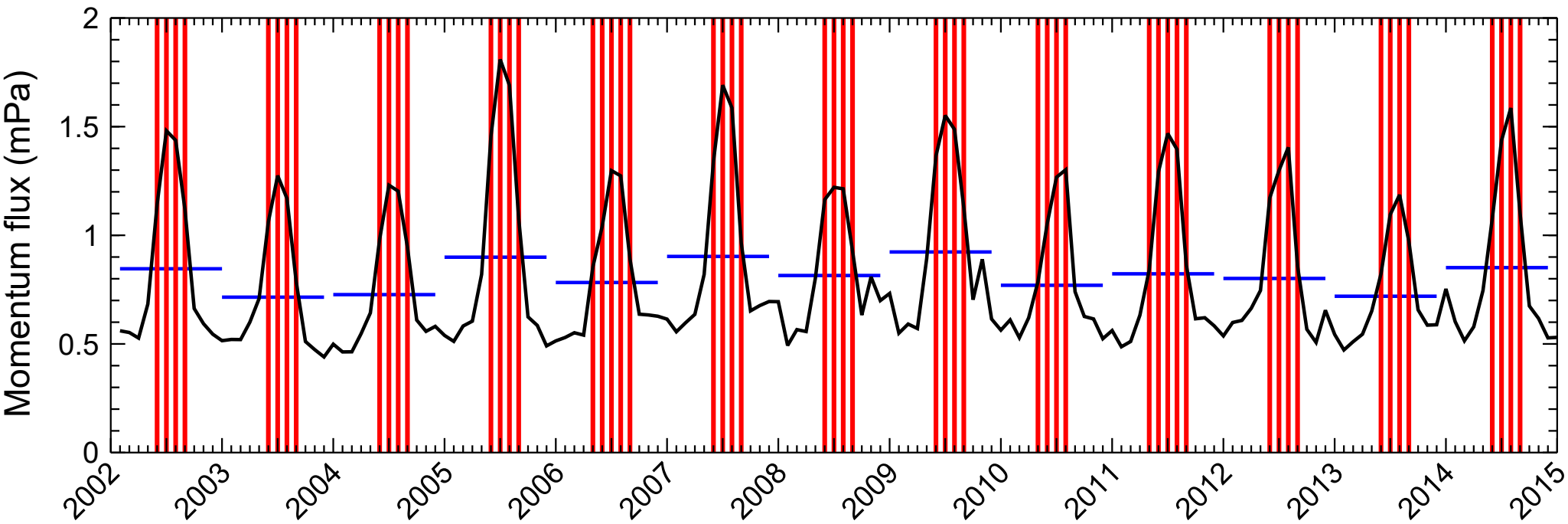
(a) Time series at 20° N
