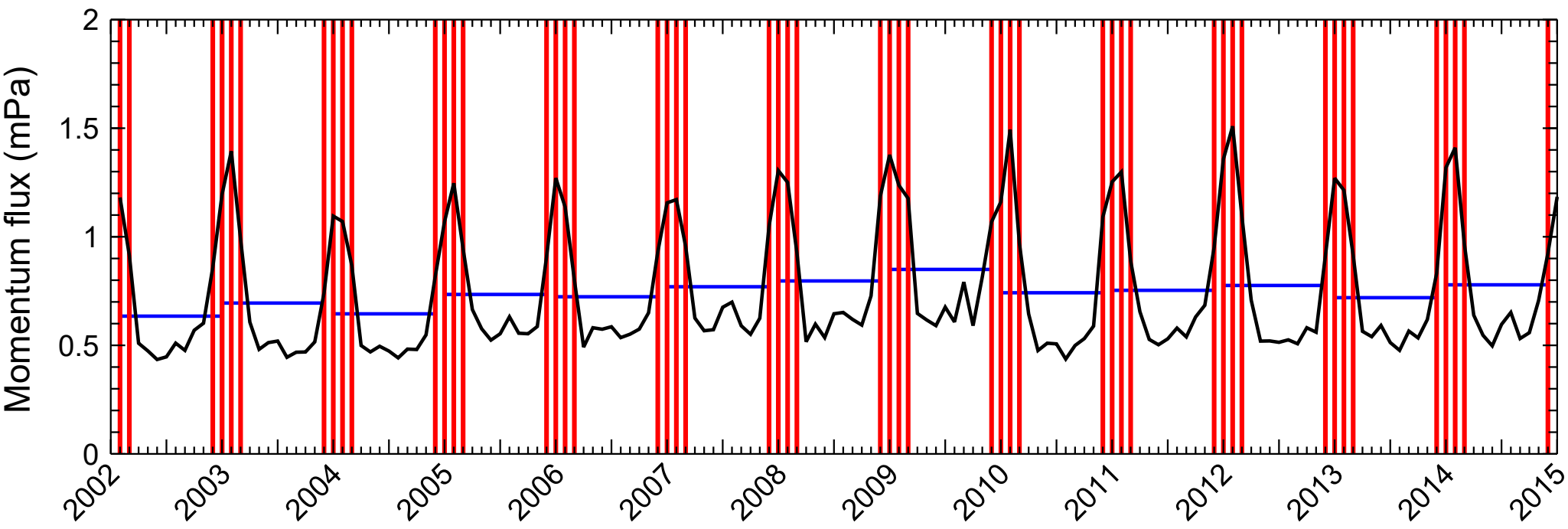
(b) Time series at 20° S
