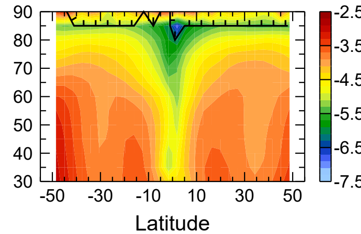
(e) AV: Zonal GWMF ( \log_{10}\text{Pa} )
