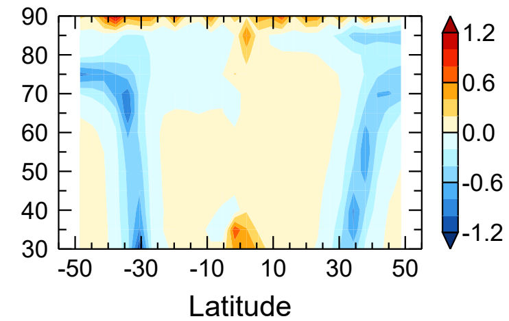
(f) AV: Difference
