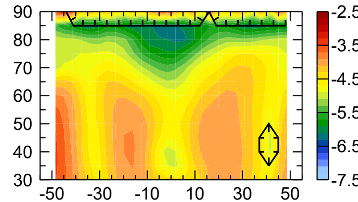
(b) SAV: Zonal GWMF ( \log_{10}\text{Pa} )
