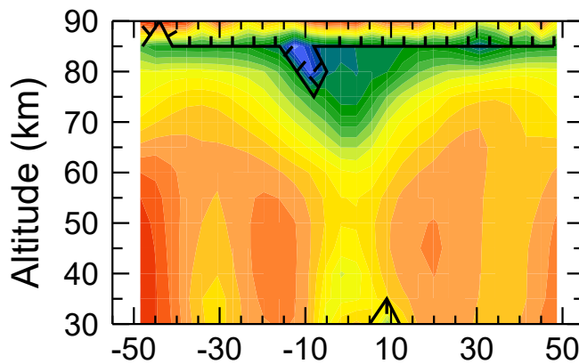
(a) SAV: |GWMF| ( \log_{10}\text{Pa} )
