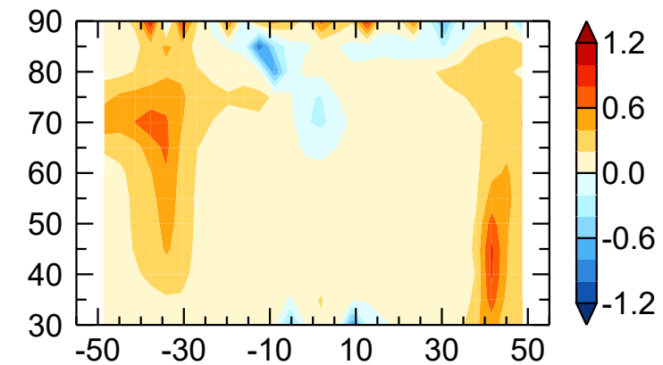
(c) SAV: Difference
