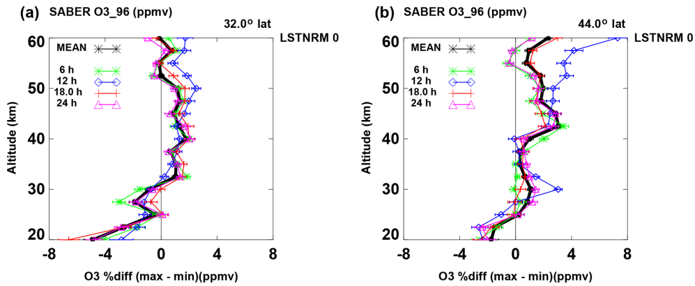
Figure A1. As in Fig. 7, ozone responses at 32° (a) and 44° from 20 to 60 km. Values are responses at solar max minus responses at solar min (%/100 sfu). Black asterisks denote our responses based on zonal means that are averages over both longitude and local time. Green asterisks denote our responses of zonal means at 6 LST, blue diamonds denote our responses of zonal means at 12 LST, red pluses denote our responses of zonal means at 18 LST, and magenta triangles denote our responses of zonal means at 24 LST, based on SABER data.
