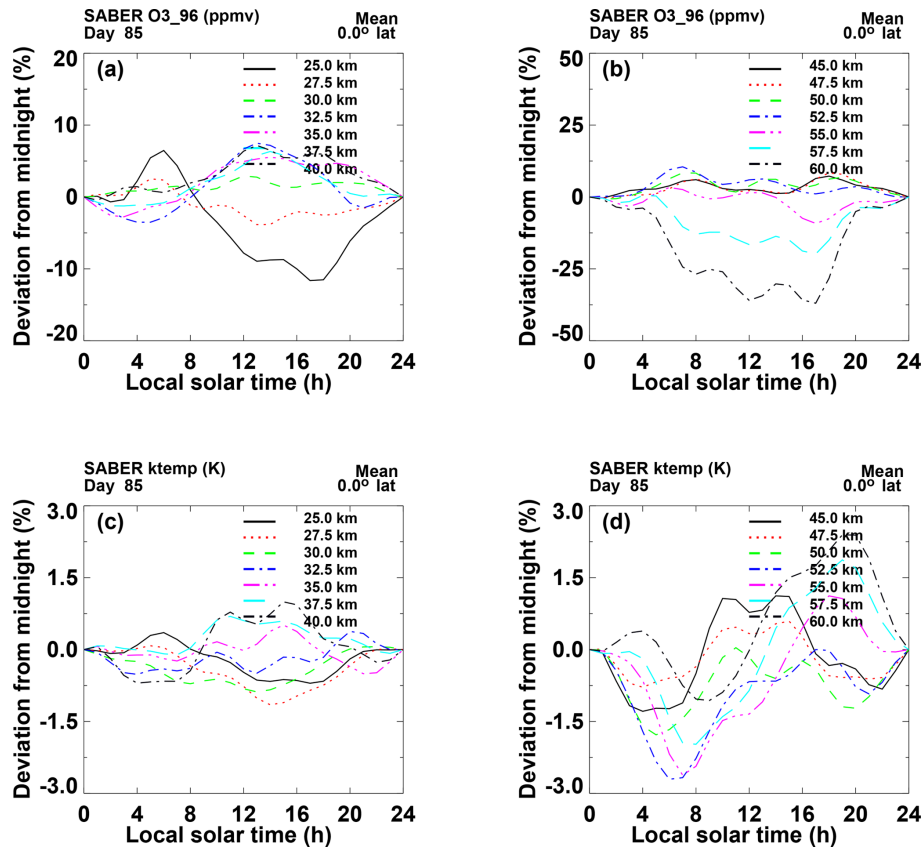
Figure 1. (a, b) Ozone zonal mean mixing ratios (ppmv) versus local time for day 05085 at the Equator. (a) At 25 to 40 km (percent deviation from midnight) and (b) 45 to 60 km. (c, d) As in (a, b), but for temperature (K).
