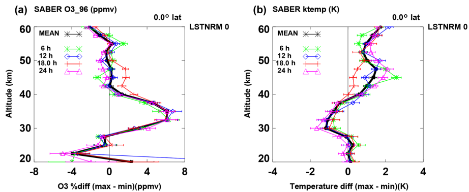
Figure 7. As in Fig. 6, but from 20 to 60 km. Ozone (a) and temperature (b) responses at 0°. Values are responses at solar max minus responses at solar min for ozone (%/100 sfu) and for temperature (K/100 sfu). Black asterisks denote our responses based on zonal means that are averages over both longitude and local time; green asterisks denote our responses of zonal means at 6 LST, blue diamonds represent responses of zonal means at 12 LST, red plusses represent responses of zonal means at 18 LST, and magenta triangles represent responses of zonal means at 24 LST, based on SABER data.
