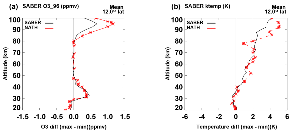
Figure 10. Ozone (a) and temperature (b) responses to solar activity versus altitude from 20 to 100 km. Values are responses at solar max minus responses at solar min (in parts per million by volume per 100 sfu for ozone and Kelvin per 100 sfu for temperature). Black lines denote SABER responses at 12° latitude; red lines denote results from Nath and Sridharan (2014) for a latitude of 10–15°, also based on SABER data.
