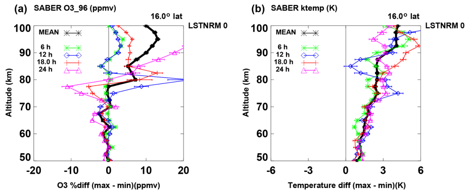
Figure 6. Ozone (a) and temperature (b) responses from 50 to 100 km at 16° N. Values are responses at solar max minus responses at solar min for ozone (%/100 sfu) and for temperature (K/100 sfu). Black asterisks denote responses based on zonal means that are averages over both longitude and local time, green asterisks denote our responses based on zonal means fixed at 6 LST, blue diamonds represent zonal means fixed at 12 LST, red plusses represent zonal means fixed at 18 LST, and magenta triangles represent zonal means fixed at 24 LST, based on SABER data.
