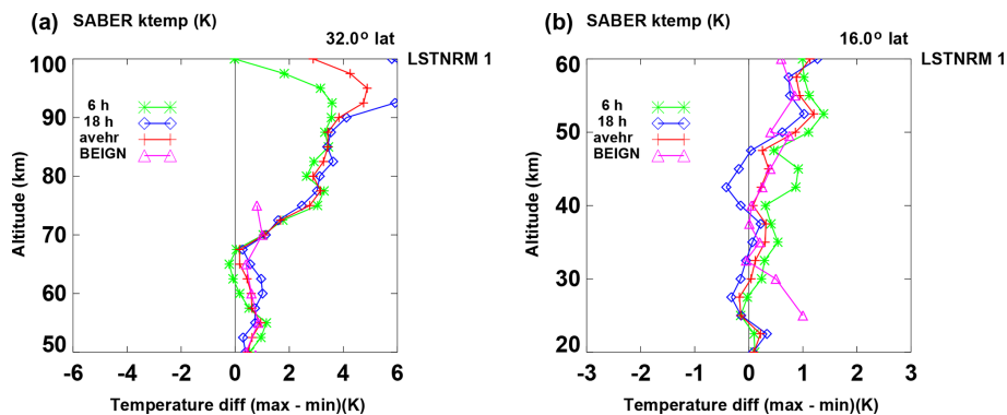
Figure 5. Corresponds to Fig. 3, but for temperature responses to solar activity versus altitude, from 50 to 100 km (a), and 20 to 60 km (b). Values are responses at solar max minus responses at solar min (K/100 sfu). Magenta triangles denote results by Beig et al. (2012), average of 6 and 18 LST (composite 0–30° N). Red plusses denote our estimate (average of 6 and 18 LST at 32° N, a and 16° N, b), based on SABER data. Green asterisks denote our estimates at 6 LST, and blue diamonds are estimates at 18 LST.
