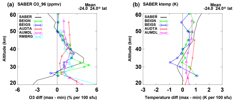
Figure 9. (a) Ozone responses versus altitude from 20 to 60 km. The black line represents SABER results averaged from 24° S to 24° N; the light blue squares denote results from Remsberg (2008, RMSBRG); the green asterisks represent Fadnavis and Beig (2006), BEIGN, 0–30° N; the blue diamonds represent BEIGs, 0–30° S, HALOE data; the red pluses denote results from Austin et al. (2008) data AUDTA; the magenta triangles represents the Austin et al. (2008) model, AUMDL, 25° S to 25° N latitude composite. (b) Temperature responses corresponding to (a).
