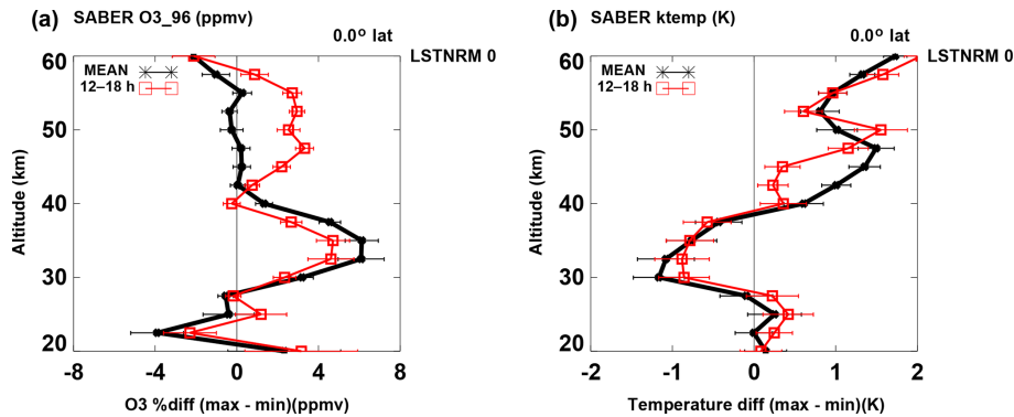
Figure 8. Ozone (a) and temperature (b) responses to solar activity versus altitude at the Equator from 20 to 60 km. Values are responses at solar max minus responses at solar min in percent per 100 sfu for ozone, and Kelvin per 100 sfu for temperature. Black asterisks denote responses based on zonal means that are averages over both longitude and local time. Red squares denote corresponding results, but with local times increasing linearly from 12 to 18 LST from 2002 to 2014.
