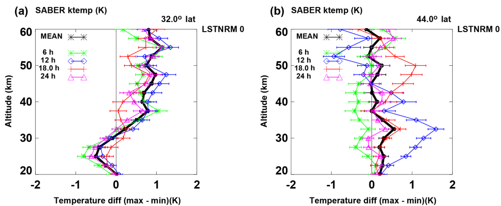
Figure A2. As in Fig. A1, but for temperature responses at 32° (a) and 44° from 20 to 60 km. Values are responses at solar max minus responses at solar min (K/100 sfu). Black asterisks denote our responses based on zonal means that are averages over both longitude and local time. Green asterisks denote our responses of zonal means at 6 LST, blue diamonds denote our responses of zonal means at 12 LST, red pluses denote our responses of zonal means at 18 LST, and magenta triangles denote our responses of zonal means at 24 LST, based on SABER data.
