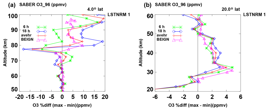
Figure 3. Ozone responses to the solar decadal cycle versus altitude at 4° N from 50 to 100 km (a), and at 20° N from 20 to 60 km (b). Values are responses at solar max minus responses at solar min (%/100 sfu). Magenta triangles denote the results from Beig et al. (2012), which are the average of responses at 6 and 18 LST (local time) and 0–30° N; red pluses denote our estimate (average at 6 and 18 LST); green asterisks denote our estimate at 6 LST; and blue diamonds denote our estimate at 18 LST.
