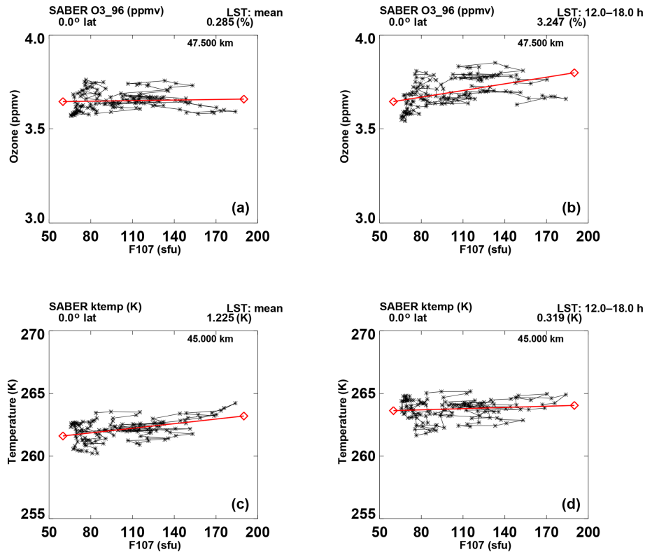
Figure 11. (a, b) Scatterplot of ozone monthly values versus 10.7 cm flux (sfu) at 47.5 km and the Equator. (a, c) Monthly values are zonal means, including the average over local time. (b, d) As in (a) and (c), but zonal means include simulated local time variations of orbital drift. (c, d) As in (a) and (b), but for temperature monthly values. Red lines represent the linear fit between LST monthly values and 10.7 cm flux. Compare with Fig. 8.
