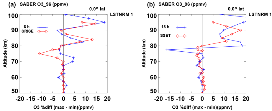
Figure 4. Ozone responses to solar activity versus altitude from 50 to 100 km at the Equator. Values are responses at solar max minus responses at solar min (%/100 sfu). Red diamonds denote results based on HALOE data from Beig et al. (2012) at 6 LST (a) and 18 LST (b), composite from 0–4° N. Blue plusses denote our results based on SABER data at 6 LST and 0° (a) and 18 LST (b).
