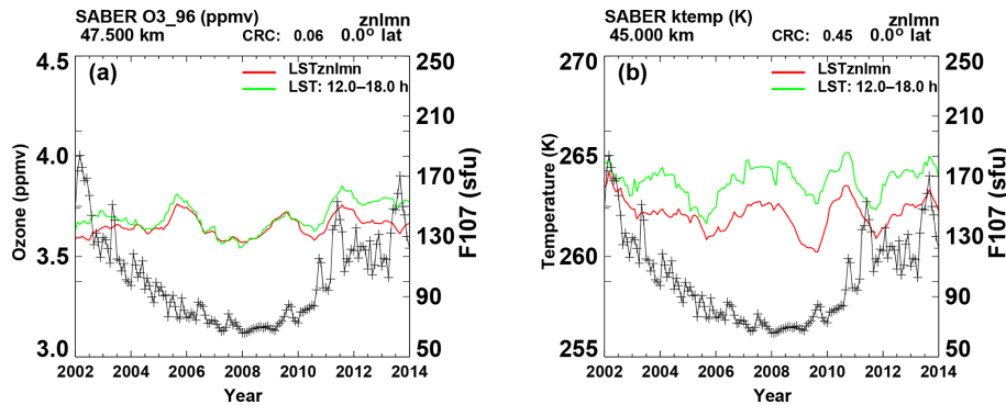
Figure 2. Ozone zonal mean mixing ratios (a, red line, ppmv) from mid 2002 to mid 2014, 47.5 km, 0°; (b), as in (a), but for temperature (K) at 45 km. The green lines represent how the data would vary if we simulated the variations with local time due to simulated orbital drifts of the NOAA operational satellites. Black lines (+, right axis) show the corresponding monthly 10.7 cm flux (sfu) provided by NOAA.
