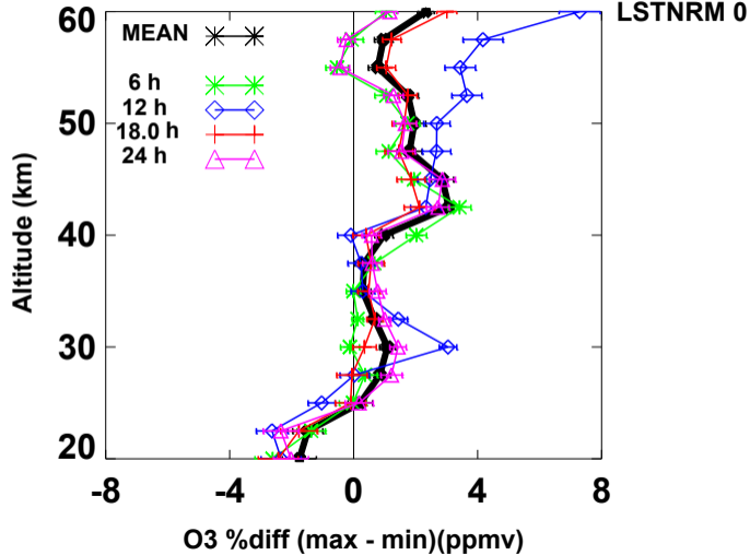
(b) SABER O3_96 (ppmv)
