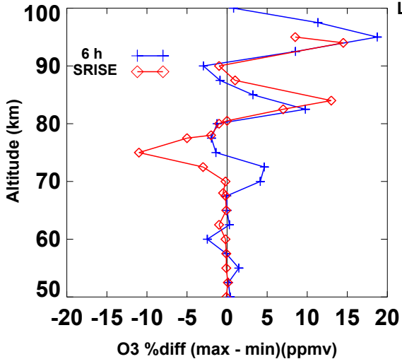
(a) SABER O3_96 (ppmv)
