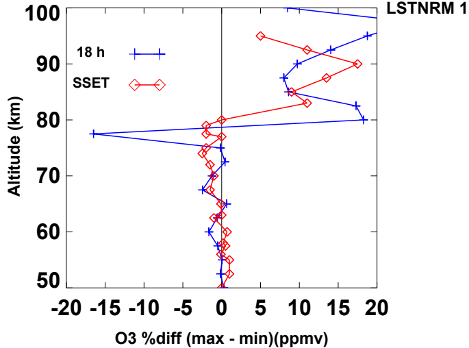
(b) SABER O3_96 (ppmv)
