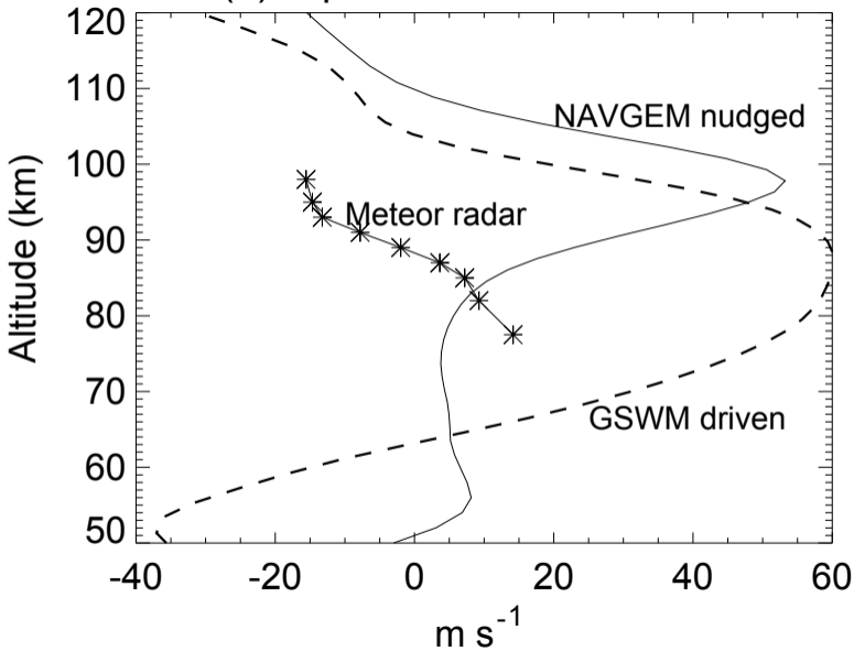
(a) Equatorial zonal mean U
