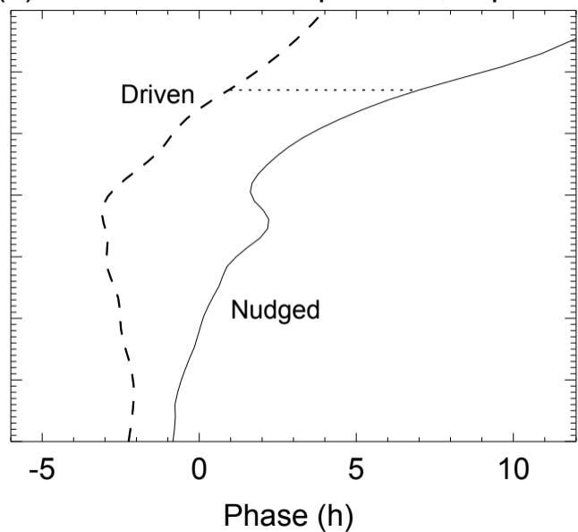
(b) Phase of SW2 temperature, Equator
