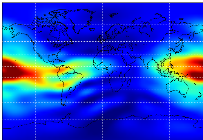
(e) 19/03/2015 02:00 UT
