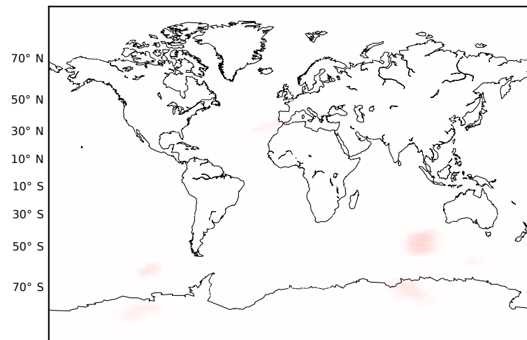
(f) 09/09/2017 02:00 UT
