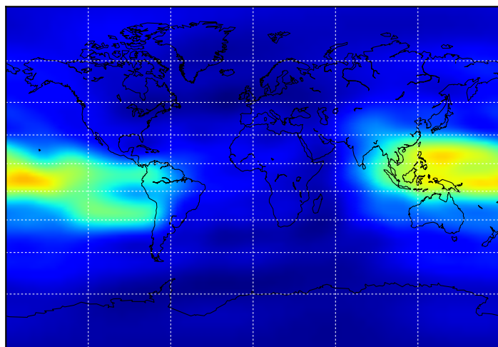
(e) 09/09/2017 02:00 UT
