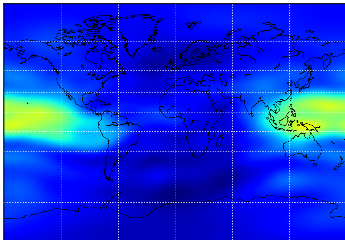
(a) 07/09/2017 02:00 UT
