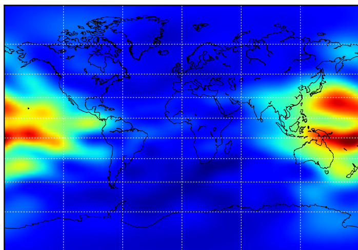
(c) 08/09/2017 02:00 UT
