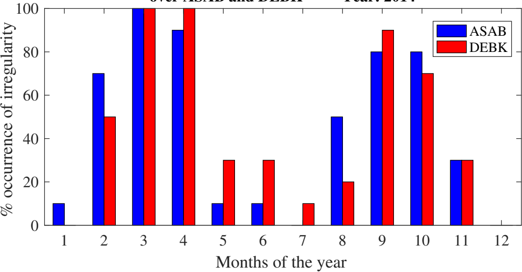
Percentage occurrence of ionospheric irregularities over ASAB and DEBK Year: 2014
