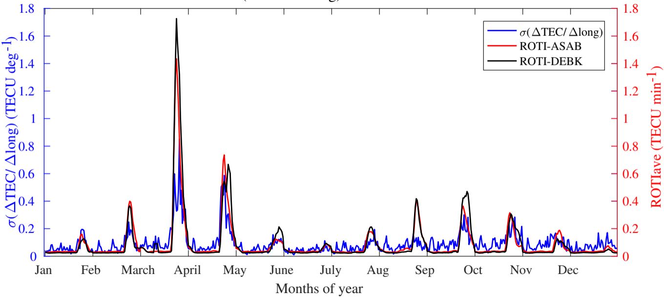
Seasonal variation of \sigma(\Delta\text{TEC}/\Delta\text{long}) and ROTI Year 2014
