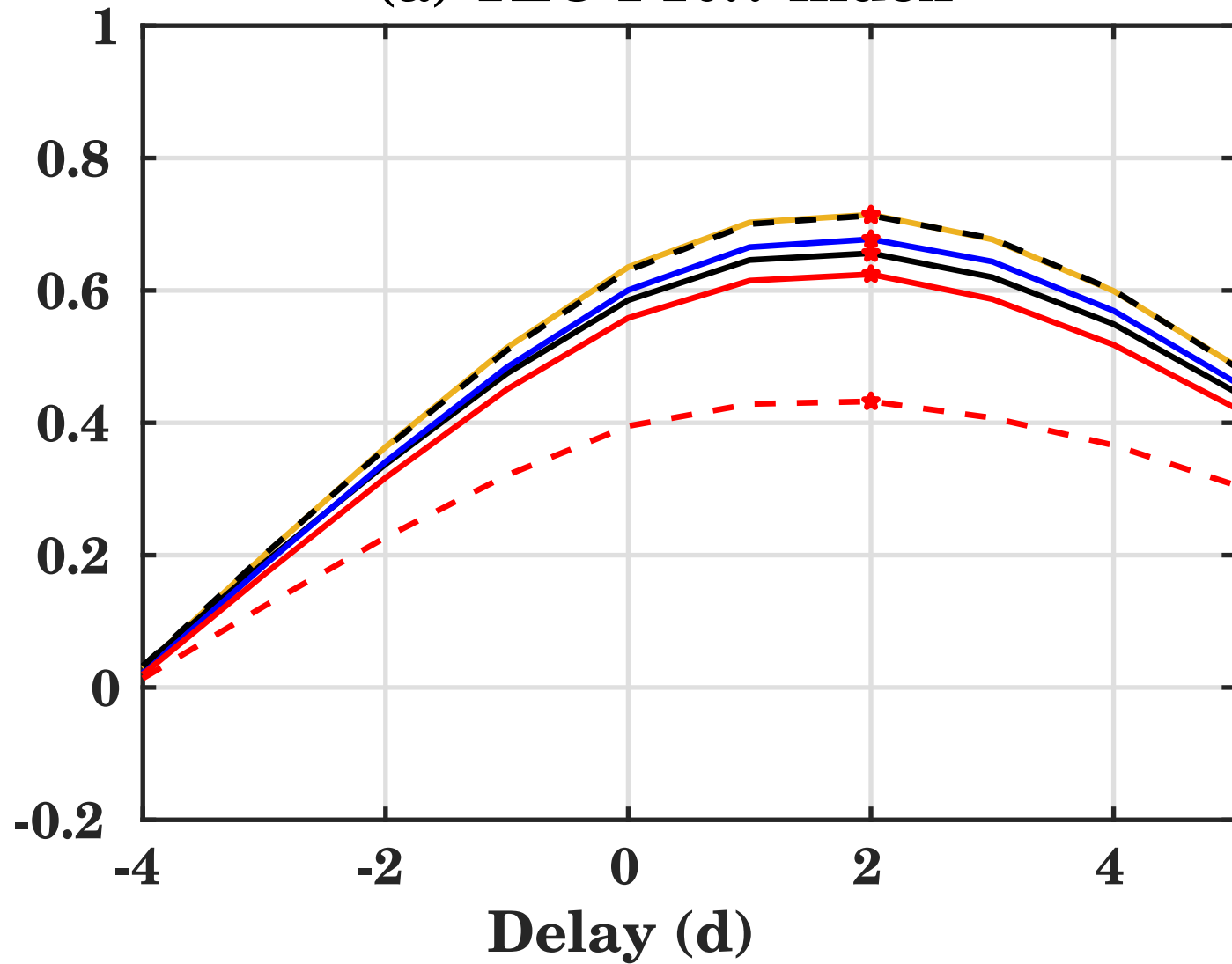
(a) TEC-F10.7 index
