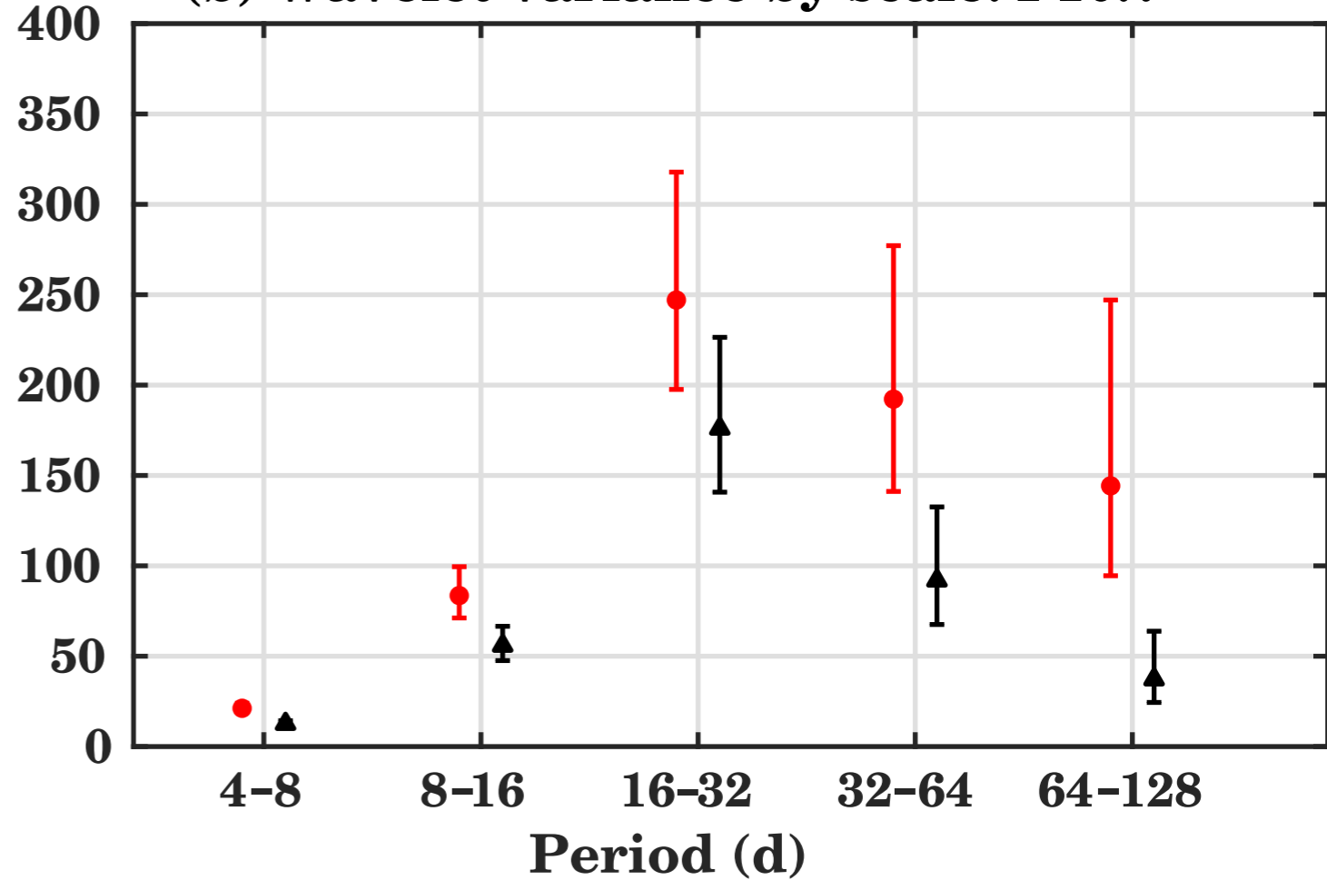
(b) Wavelet variance by scale: F10.7
