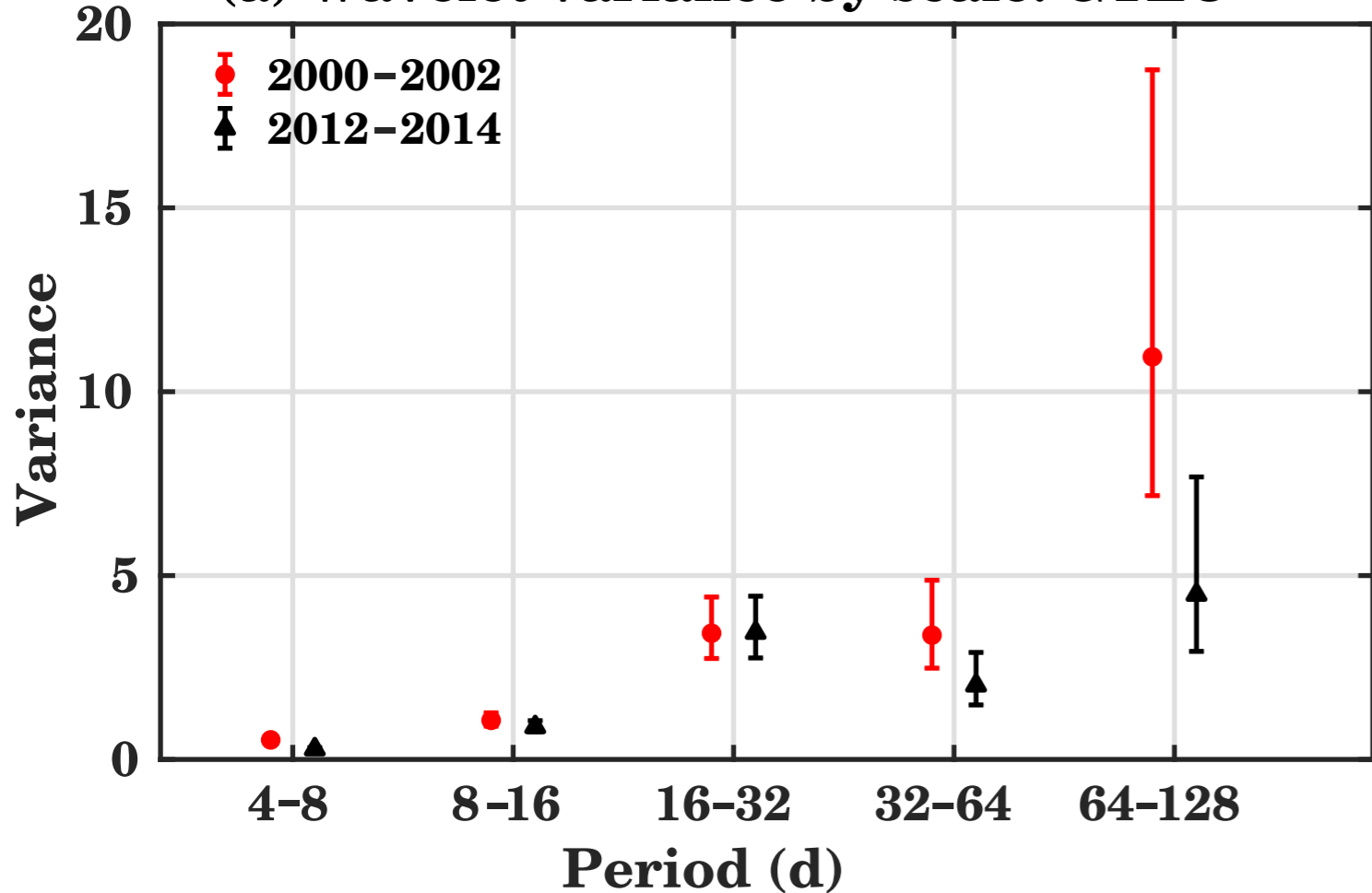
(a) Wavelet variance by scale: GTEC
