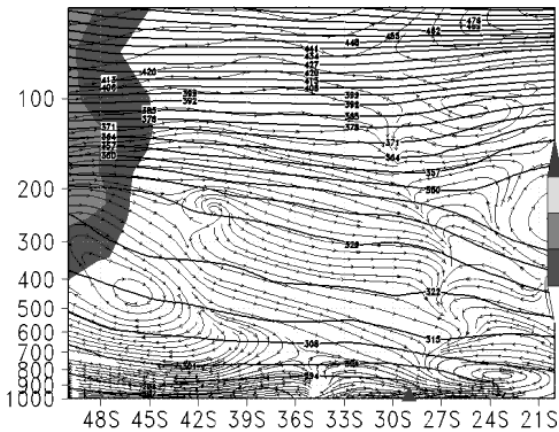
Potential temperature (K) and wind (m s -1 )
