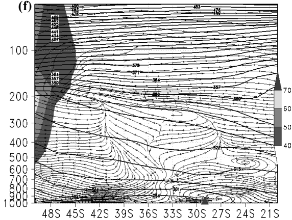
Potential temperature (K) and wind (m s -1 )
