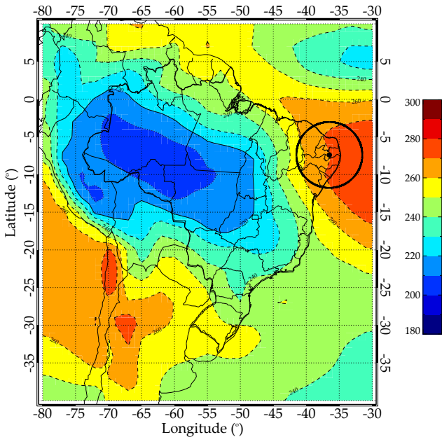
OLR ( W m^{-2} ) - Summer (Nov–Feb)
