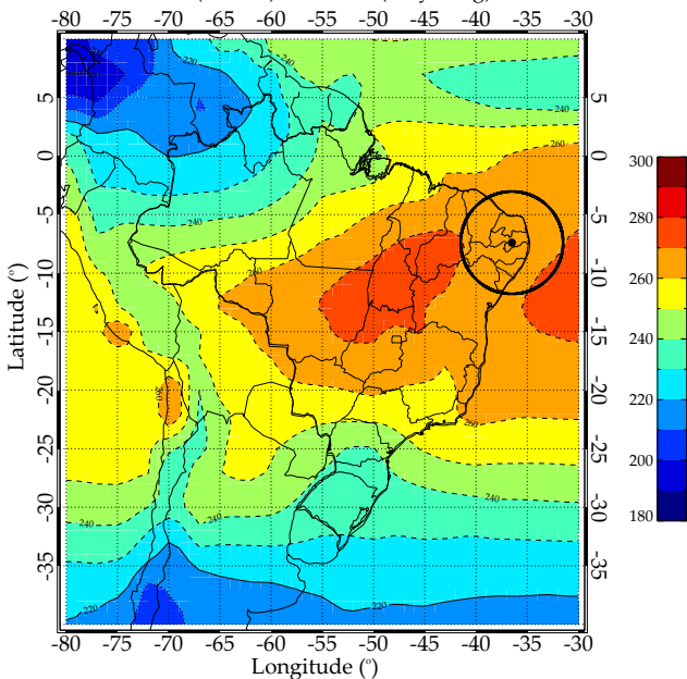
OLR ( W m^{-2} ) - Winter (May–Aug)
