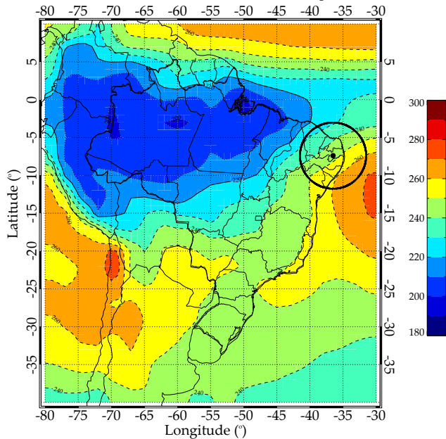
OLR ( W m^{-2} ) - Autumn (Mar–Apr)
