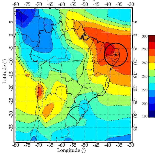
OLR ( W m^{-2} ) - Spring (Sep–Oct)
