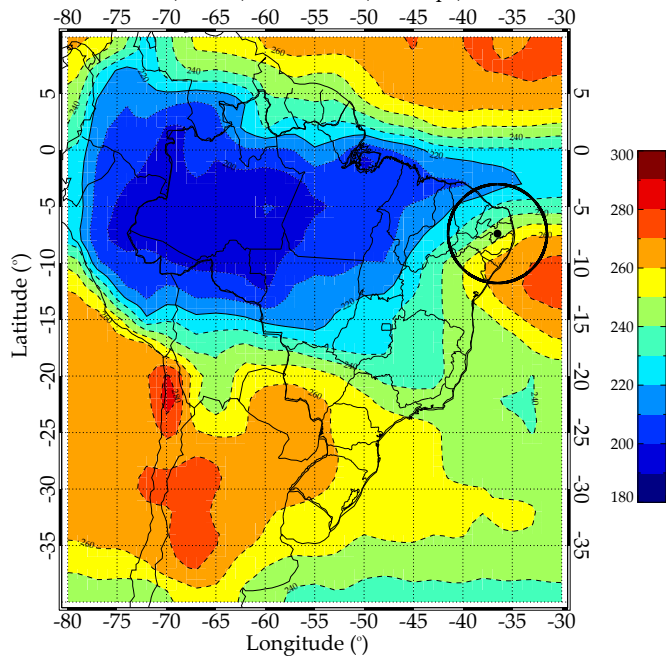
OLR ( W m^{-2} ) - Autumn (Mar-Apr) - 2009
