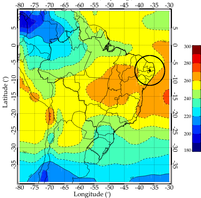
OLR ( W m^{-2} ) - Winter (May-Aug.) - 2009
