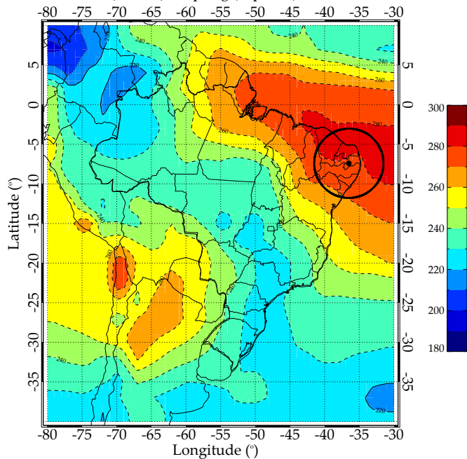
OLR ( W m^{-2} ) - Spring (Sep-Oct) - 2009
