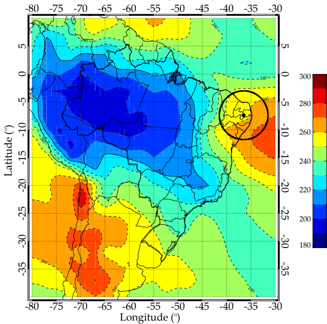
OLR ( W m^{-2} ) - Summer (Nov-Feb) - 2009
