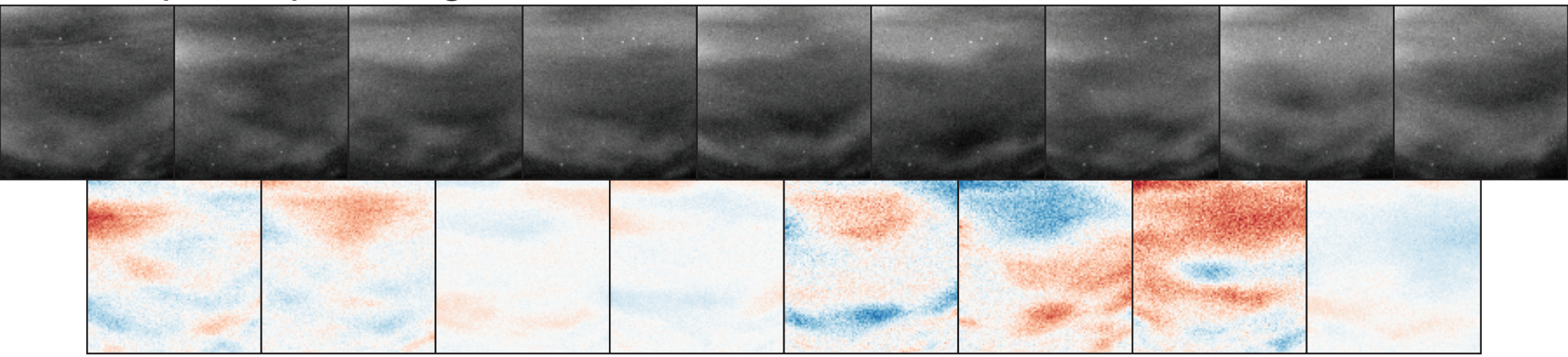
(c) Amorphous pulsating aurora (APA)
