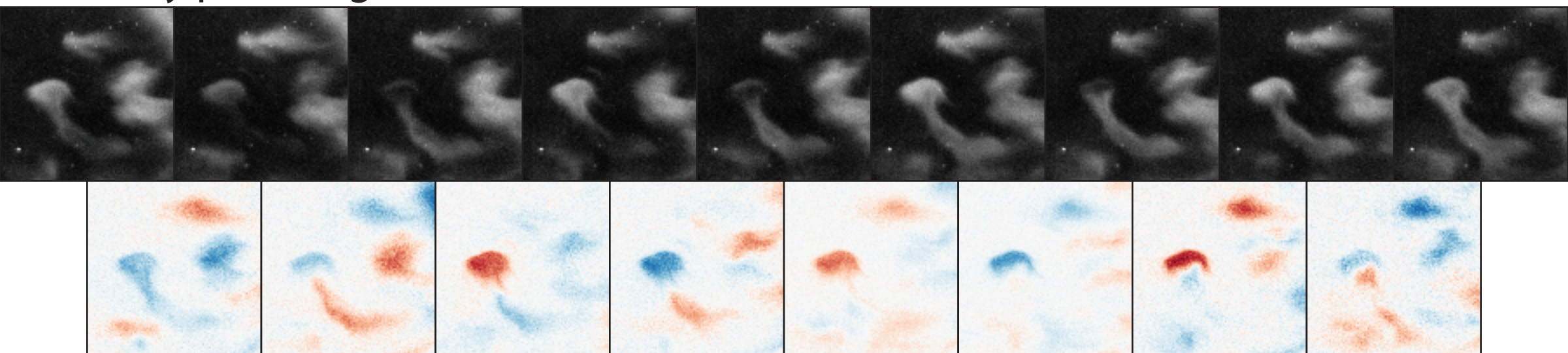
(b) Patchy pulsating aurora (PPA)
