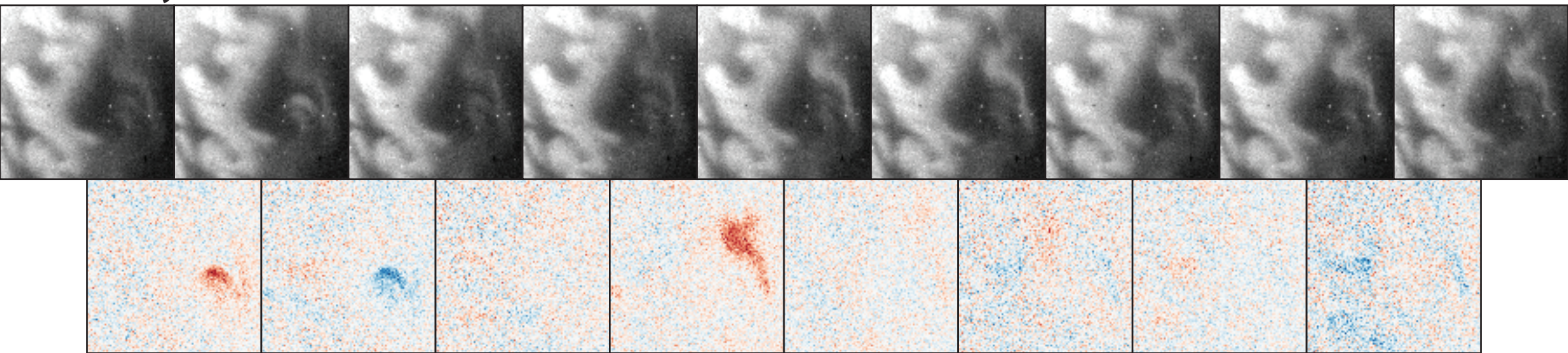
(a) Patchy aurora (PA)
