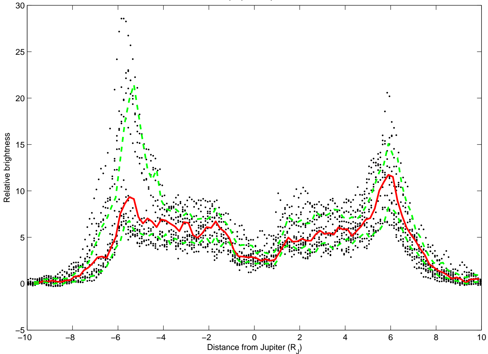
Superposed epoch
