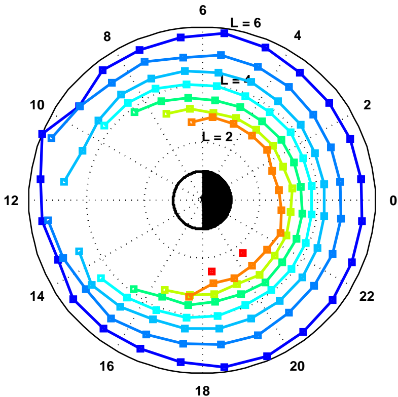
(a) Swarm SSFAC boundary
